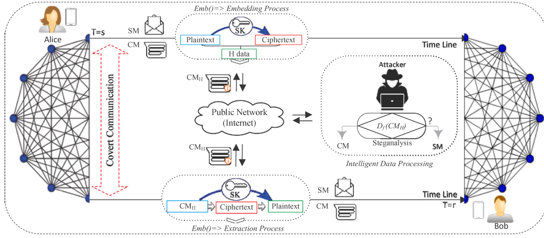
Fig. 1. A potential covert communication scenario in which Alice and Bob utilize a text steganography approach when sending ( s ) or receiving ( r ) a CM_H considering an access delay between two parties, denoted as the T(s, r) .
