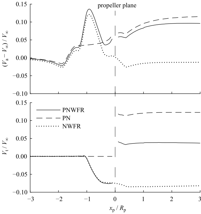
Fig. 10. For three configurations, PNWFR, PN and NWFR, the radially and circumferentially averaged axial and tangential velocity distribution through the left propeller approximate streamtube is plotted in cruise. The streamtube was approximated by a cylinder of radius equal to the propeller radius from 3 radii upstream to 3 radii downstream of the propeller.
