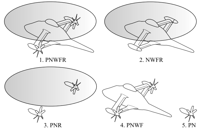
Fig. 2. The five different simulated configurations including labels (P: propeller; N: nacelle; W: wing; F: fuselage; R: rotor).
