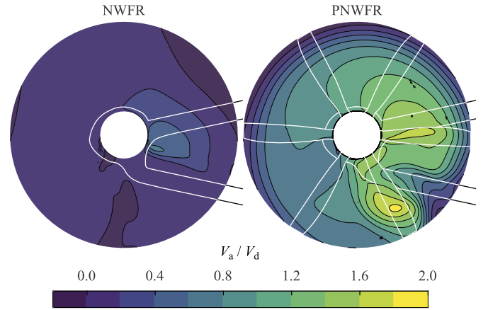
Fig. 19. Time-averaged axial velocity component is plotted on the plane visualised in Fig. 15, upstream of the left propeller in hover. The effect of the propeller is shown by means of comparison of the NWFR and PNWFR configuration.
