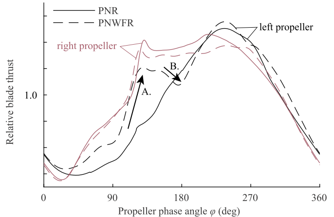
Fig. 17. Blade thrust is plotted relative to the time-averaged blade thrust during a full rotation in hover for the PNR and PNWFR configuration. Phase angle \varphi is defined in Fig. 1 and the quantities are plotted divided through the PNWFR time-averaged value. Annotation A. indicates the effect of the wake of the wings and nacelle and B. the effect of main rotor downwash deflected by the upper wing.
