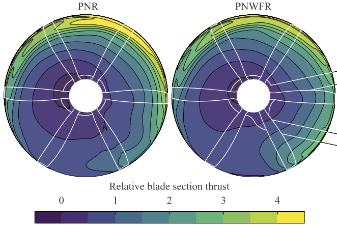
Fig. 18. The blade section thrust relative to the time-averaged blade thrust is plotted for each circumferential position of the left propeller in hover. The effect of the wings is shown by means of comparison of the PNR and PNWFR configuration at equal blade pitch angle.
