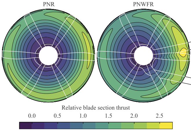
Fig. 6. The blade section thrust relative to the time-averaged blade thrust is plotted for each circumferential position of the left propeller in cruise. The effect of the wings is shown by means of comparison of the PNR and PNWFR configuration.
