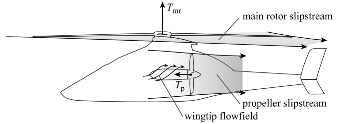
Fig. 4. Sketch of main rotor, box-wing and propeller aerodynamic interaction in cruise, indicating the direction of the main rotor thrust T_{mr} and propeller thrust T_p .
