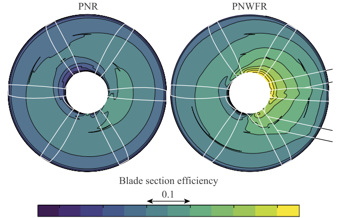
Fig. 8. The blade section efficiency T'V_\infty/P' is plotted for each circumferential position of the left propeller in cruise. The effect of the wings is shown by means of comparison of the PNR and PNWFR configuration.
