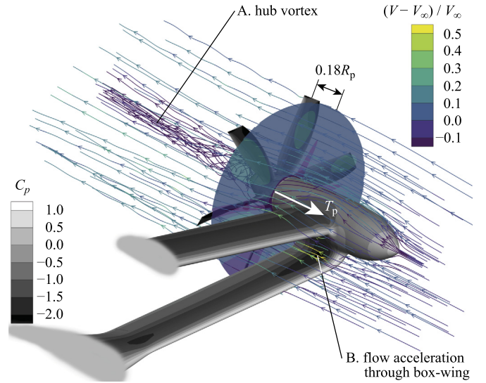
Fig. 5. For the PNWFR configuration in cruise, the flowfield is visualised through the left propeller, with velocity contours on streamtraces and on a plane 0.18R_p upstream of the propeller. Only the left box-wing, nacelle and propeller are shown, marked with contours of the pressure coefficient C_p = (p - p_\infty)/q_\infty .
