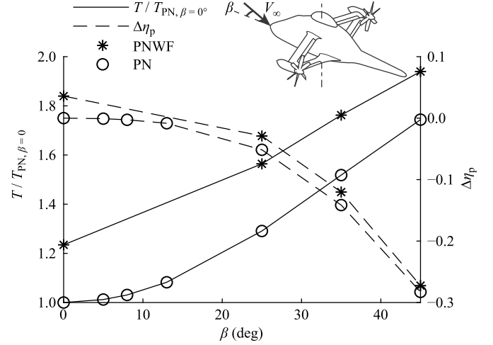
Fig. 13. Right propeller thrust T and propulsive efficiency \eta_p = (TV_\infty \cos \beta) / P are plotted against sideslip \beta at constant blade pitch angle for a reduced cruise speed for manoeuvring of V_\infty = 140 kt (72.0 m/s). A comparison is shown between the PNWF and PN configuration and quantities are with respect to PN configuration quantities at zero sideslip.
