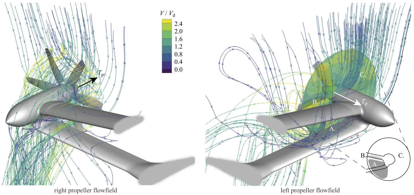
Fig. 15. For the PNWFR configuration in hover, the flow through the propellers is visualised, with velocity contours on streamtraces and on a plane 0.18R_p upstream of the left propeller. The fuselage is not shown. Annotation A. indicates the wake of the wings and nacelle, B. main rotor downwash deflected by upper wing and C. the area undisturbed by the wings.
