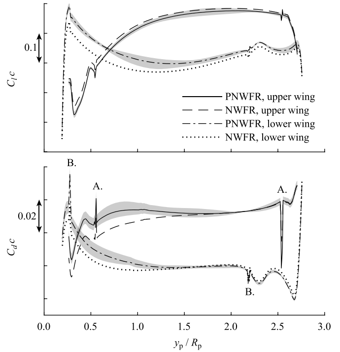
Fig. 11. Time-averaged wing loading comparison between PNWFR and NWFR configuration for the left wing in cruise, with coordinate y_p as defined in Fig. 1 and c the wing chord. Shaded area indicates time-variation. Annotation A. and B. indicate the effect of the upper and lower wing flap edge gap.
