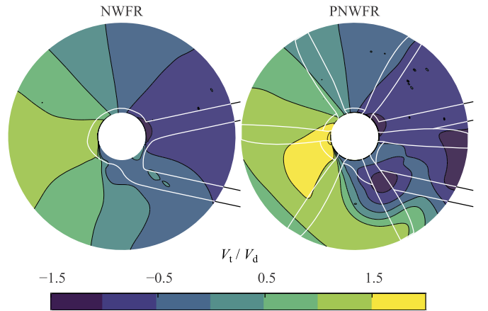
Fig. 20. Time-averaged tangential velocity component is plotted corresponding to Fig. 19.
