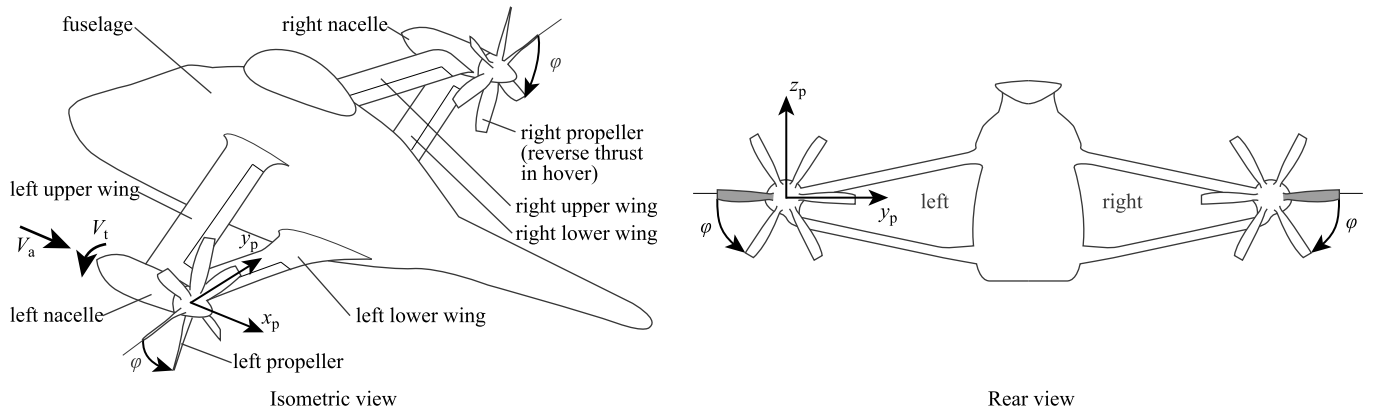
Fig. 1. Sketches of the Airbus RACER without main rotor and tailplanes. Propeller blade phase angle \phi and axial and tangential velocity components V_a and V_t are indicated.
