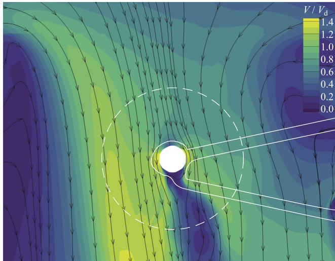
Fig. 16. The velocity field in a plane through the left propeller in hover is shown for the NWFR configuration, so without propeller present.
