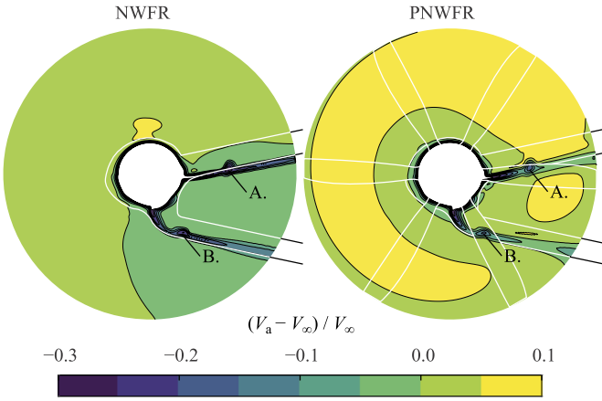
Fig. 7. Time-averaged axial velocity component is plotted on the plane visualised in Fig. 5, upstream of the left propeller in cruise. The effect of the propeller is shown by means of comparison of the NWFR and PNWFR configuration. Annotation A. and B. indicate the effect of the upper and lower wing flap edge gap.
