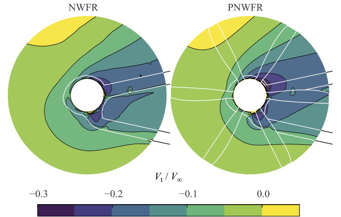
Fig. 9. Time-averaged tangential velocity component is plotted on the plane visualised in Fig. 5, upstream of the left propeller in cruise. The effect of the propeller is shown by means of comparison of the NWFR and PNWFR configuration.
