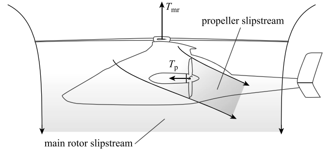
Fig. 14. Sketch of main rotor and propeller aerodynamic interaction in hover, indicating the direction of the main rotor thrust T_{mr} and propeller thrust T_p .
