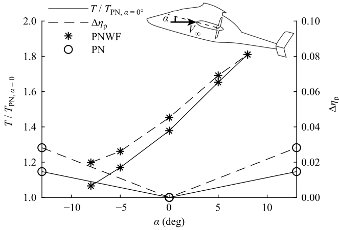
Fig. 12. Left propeller thrust T and propulsive efficiency \eta_p = (TV_\infty \cos \alpha) / P are plotted against angle of attack \alpha at constant blade pitch angle for V_\infty = 220 kt (113.2 m/s). A comparison is shown between the PNWF and PN configuration and quantities are with respect to PN configuration quantities at zero angle of attack.
