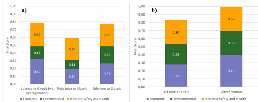
Figure 2: Comparative Results of the ‘Green-by-Design method’ of the two case studies: a) ethylene glycol production; b) fava bean protein isolate production. The final score can vary between 0 and 1 and the higher the final score, the higher is the sustainability potential of the design concept under evaluation.
