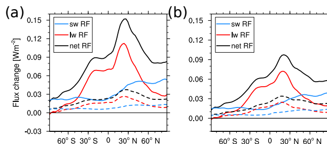
Figure 9. Zonal mean of shortwave, longwave, and net radiative \text{O}_3 forcing of (a) land transport and (b) ship traffic. The continuous lines give the results of the tagging method, and the dashed lines of the perturbation method.
