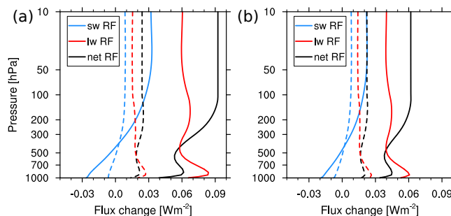
Figure 10. Vertical profile of globally averaged shortwave, longwave, and net radiative \text{O}_3 forcing of (a) land transport and (b) ship traffic. The continuous lines give the results of the tagging method, and the dashed lines of the perturbation method.
