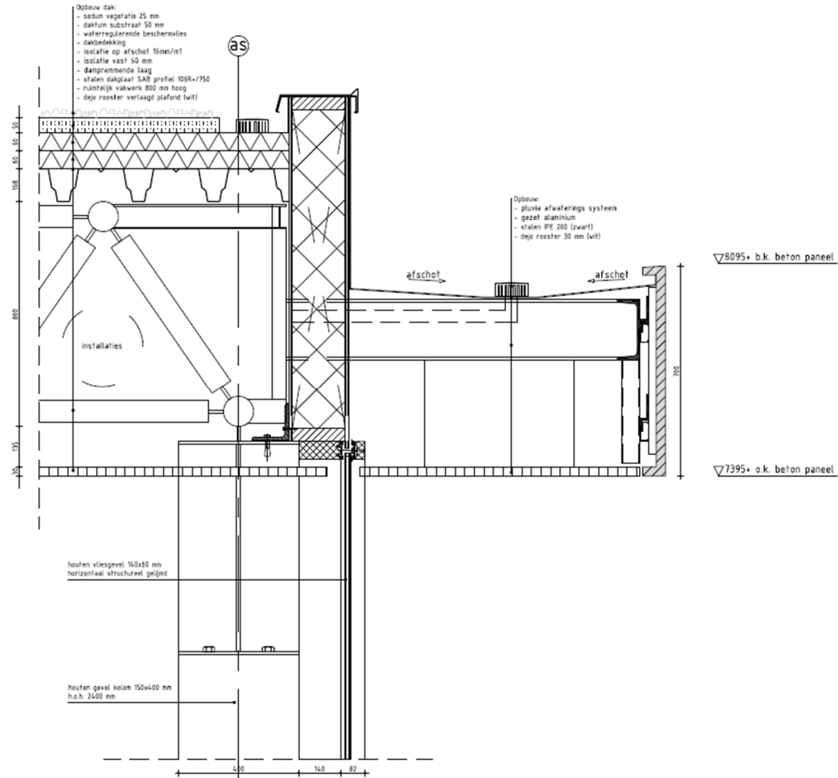
Science Business Center - dakrand detail
