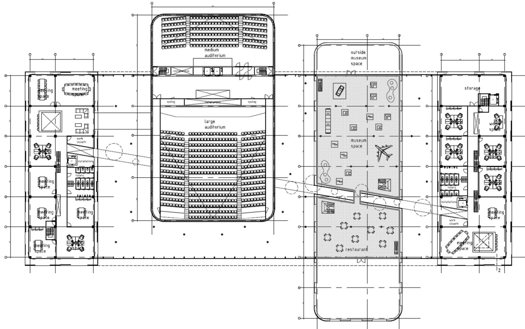
Science Business Center - plattegrond 1 ste verdieping
