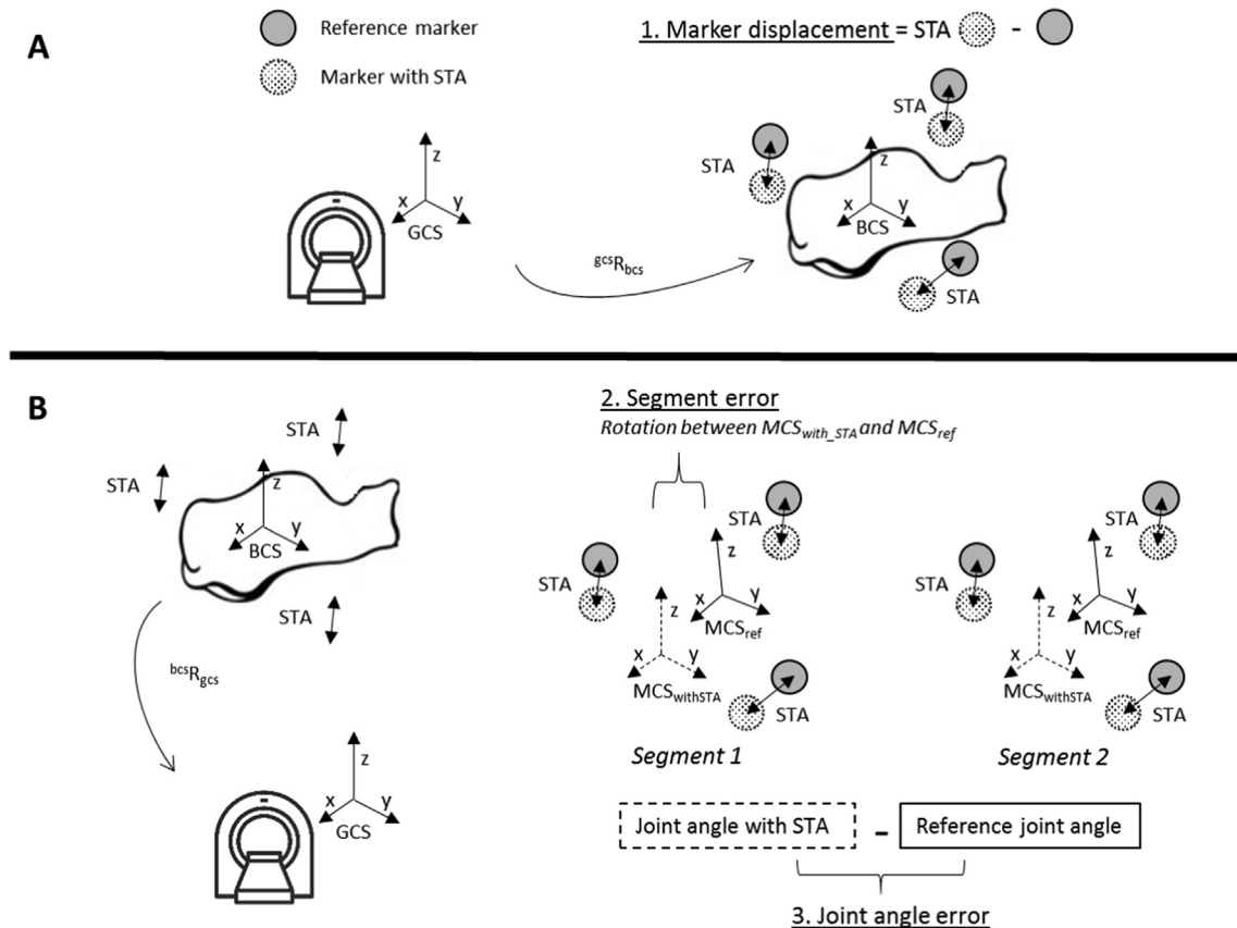
Fig. 3. Schematic overview of the data analysis to calculate (A) the 3D marker displacements (i.e. STAs) and (B) the error in segment orientation and joint angle due to STAs. Abbreviations: GCS: global coordinate system; BCS: bone coordinate system; {}^{GCS}R_{BCS} : rotation matrix from GCS to BCS; MCS_{ref} : marker coordinate system based on reference marker positions (solid). MCS_{with\_STA} : marker coordinate system based on marker positions with STAs (dashed); {}^{GCS}R_{BCS} : rotation matrix from BCS to GCS.
