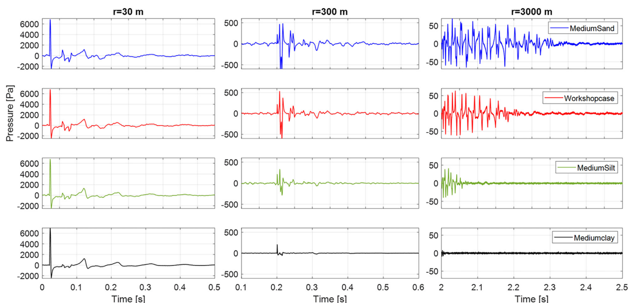
FIG. 6. (Color online) Sound pressures at 30 m (left), 300 m (middle), and 3000 m (right) for different sediment types.
