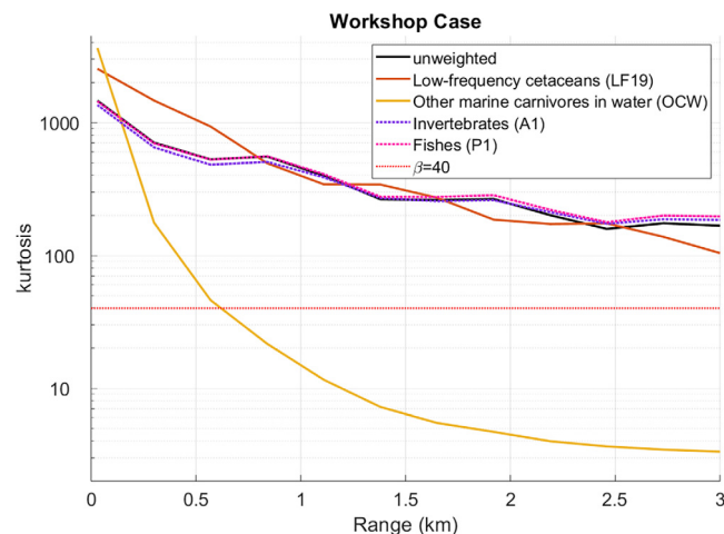
FIG. 12. (Color online) Range variation of kurtosis for the marine mammal auditory frequency weighting functions from Table IV. The red dotted line is the kurtosis value of 40. T = 10 s.
