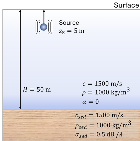
FIG. 2. (Color online) Problem geometry. Adapted from Fig. 1 of Ainslie et al. (2024).
