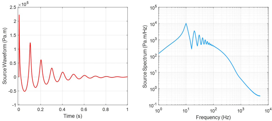
FIG. 1. (Color online) Airgun source waveform (left) and spectrum (right).
