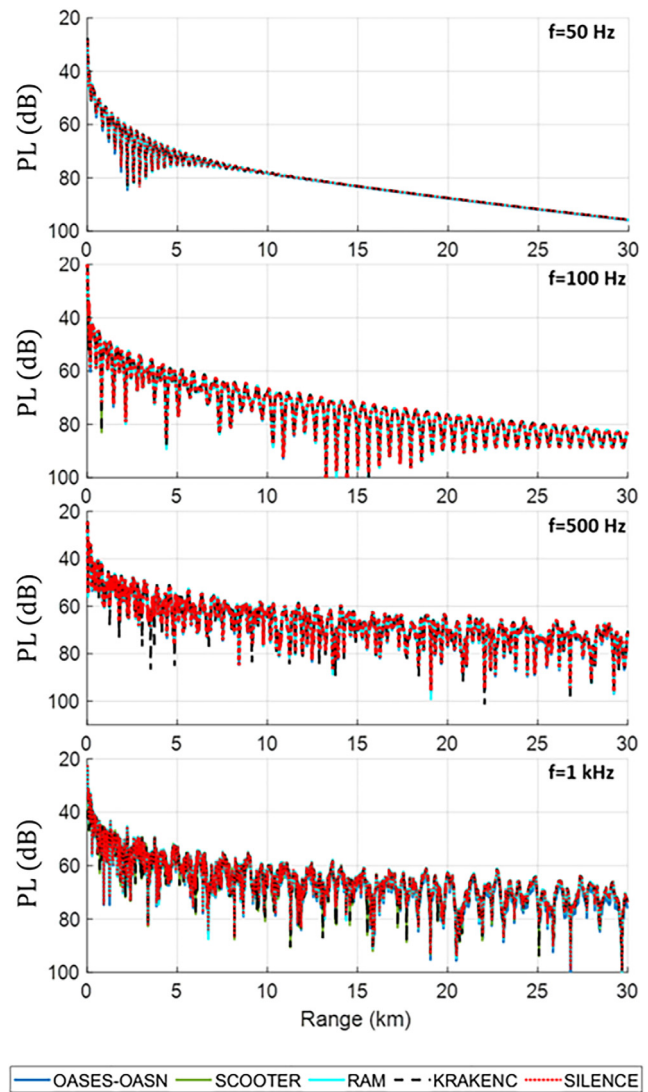
FIG. 3. (Color online) Comparison of propagation loss (PL) [re 1 m 2 (dB)] results of SILENCE with other models at 50, 100, 500, and 1000 Hz.
