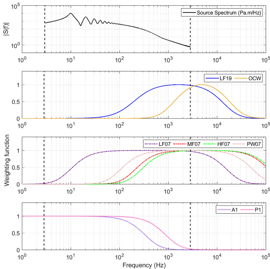
FIG. 11. (Color online) The source spectrum of single airgun (top). The lower graphs show the auditory frequency weighting functions across frequency from Southall et al. (2019), Southall et al. (2007), and Lucke et al. (2024).
