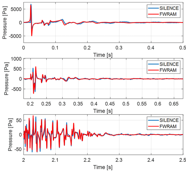
FIG. 4. (Color online) Comparison of the time domain waveforms calculated with different propagation models (SILENCE and FWRAM). Shown is sound pressure vs time for ranges 30 m (upper), 300 m (middle), and 3000 m (lower).
