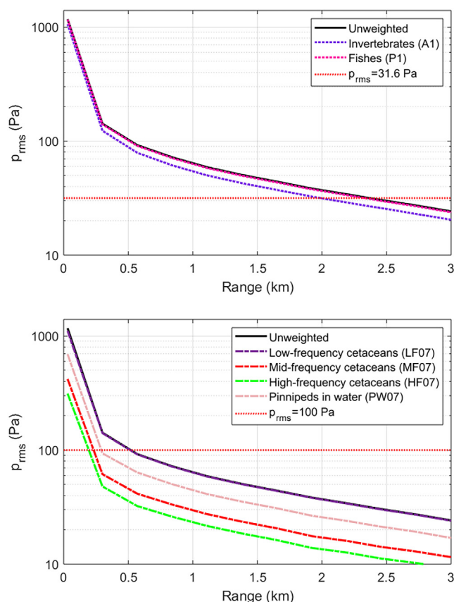
FIG. 13. (Color online) Range variation of rms sound pressure for different auditory weighting functions from Lucke et al. (2024) (top) for fishes and invertebrates and Southall et al. (2007) (bottom) for marine mammals. More details about the invertebrates and fishes are given in Table III. Sediment properties for the JAM Workshop case are used. T=0.1 s. The rms sound pressure thresholds for behavioural effects are 31.6 Pa for fishes and 100 Pa for mammals (NMFS, 2023).
