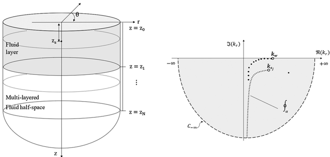
FIG. 14. Schematic depiction of the Pekeris waveguide in cylindrical coordinate (left) and visualization of complex wavenumber integration approach based on the EJP branch cut for the Pekeris waveguide (right).
