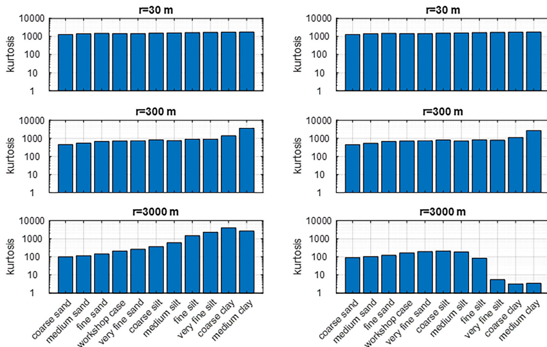
FIG. 8. (Color online) Kurtosis with (right) and without (left) additional Gaussian noise at 30, 300, and 3000 m for different sediment types. T = 10 s. The frequency band is between 2.818 Hz and 2818 Hz (band 1 in Table III).
