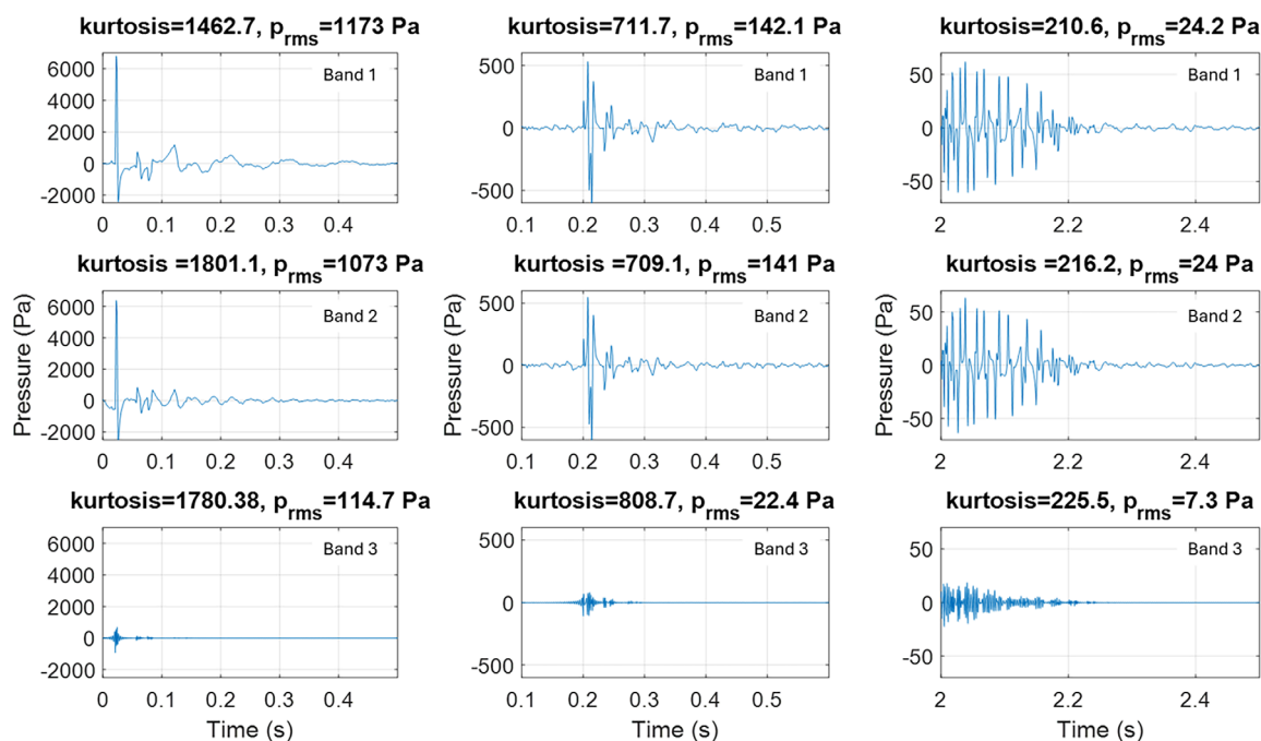
FIG. 5. (Color online) Time distribution calculations for different bandwidths. The sediment parameters from the workshop case are used. The minimum and maximum frequencies are listed in Table III.
