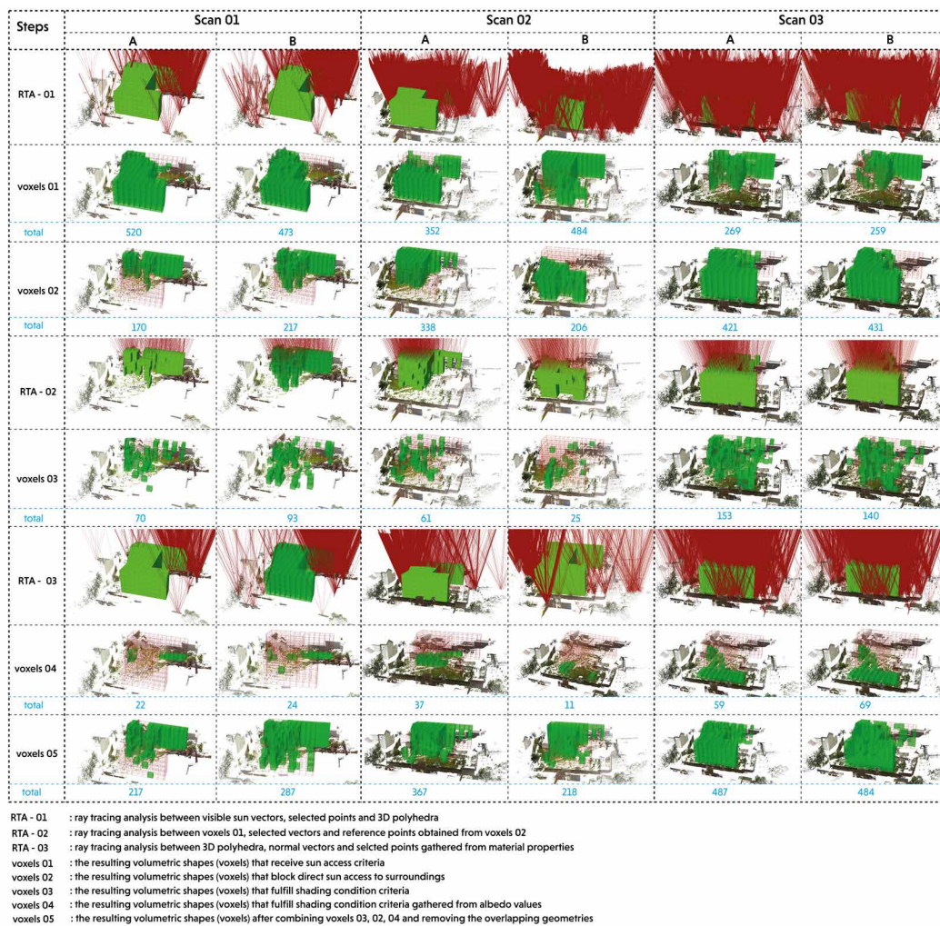
FIG. 5.27 The geometric configuration of subtractive shading envelopes based on sequential steps of design simulation.
