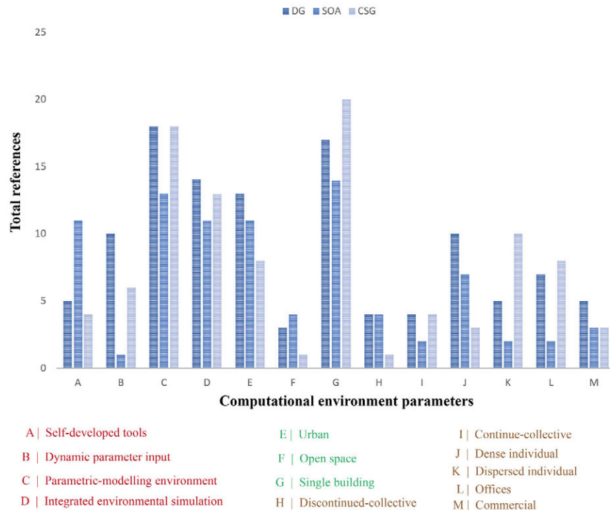
FIG. 2.5 Distribution of computational environment parameters according to the corresponding computational methods
