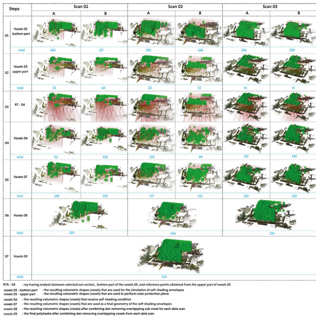
FIG. 5.28 Geometric configuration of subtractive shading envelopes
