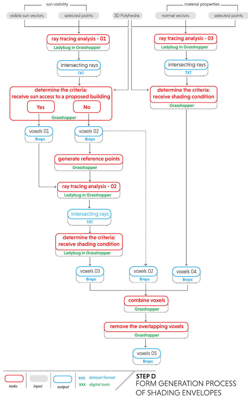
FIG. 5.19 Detailed procedures for the design simulation.
