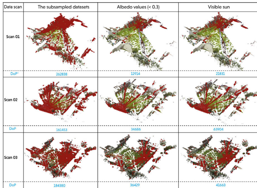
FIG. 5.26 The resulting points after performing the selection criteria
