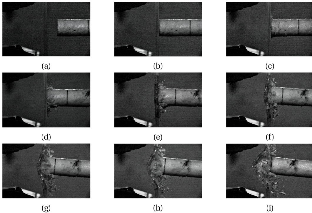
Fig. 14. Deformation of an intact CS1 laminated glass specimen (test type D, in elevation) at different time stamps during impact with a polymer projectile: (a) projectile arriving at target, (b) t = 0 \mu\text{sec} , (c) t = 250 \mu\text{sec} , (d) t = 687.5 \mu\text{sec} , (e) t = 875 \mu\text{sec} , (f) t = 1187.5 \mu\text{sec} , (g) t = 1437.5 \mu\text{sec} , (h) t = 1562.5 \mu\text{sec} and (i) t = 1937.5 \mu\text{sec} .
