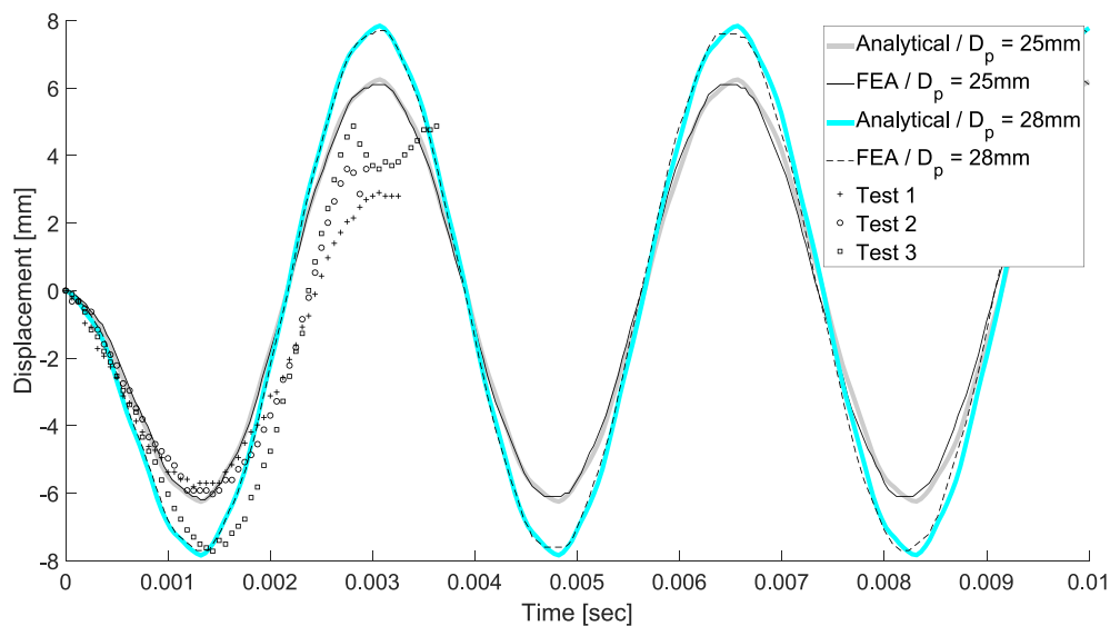
Fig. 9. Comparison of theoretical predictions (analytical and FEA) with the experimentally recorded (Tests 1–3) mid-span displacement time-history of aluminium specimens impacted by foam projectiles.
