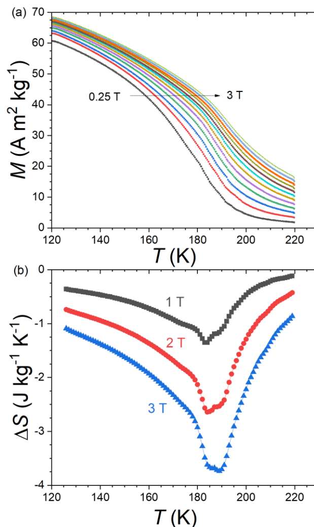
Figure 7. Magnetocaloric effect of \text{MnFe}_{0.53}\text{Ni}_{0.47}\text{Si}_{0.94}\text{Al}_{0.06} quenched from 1100^\circ\text{C} : (a) M(T) curves recorded upon heating in different magnetic fields (heating rate = 1 \text{ K min}^{-1} ); (b) isothermal entropy change calculated from M(T) curves upon heating.
