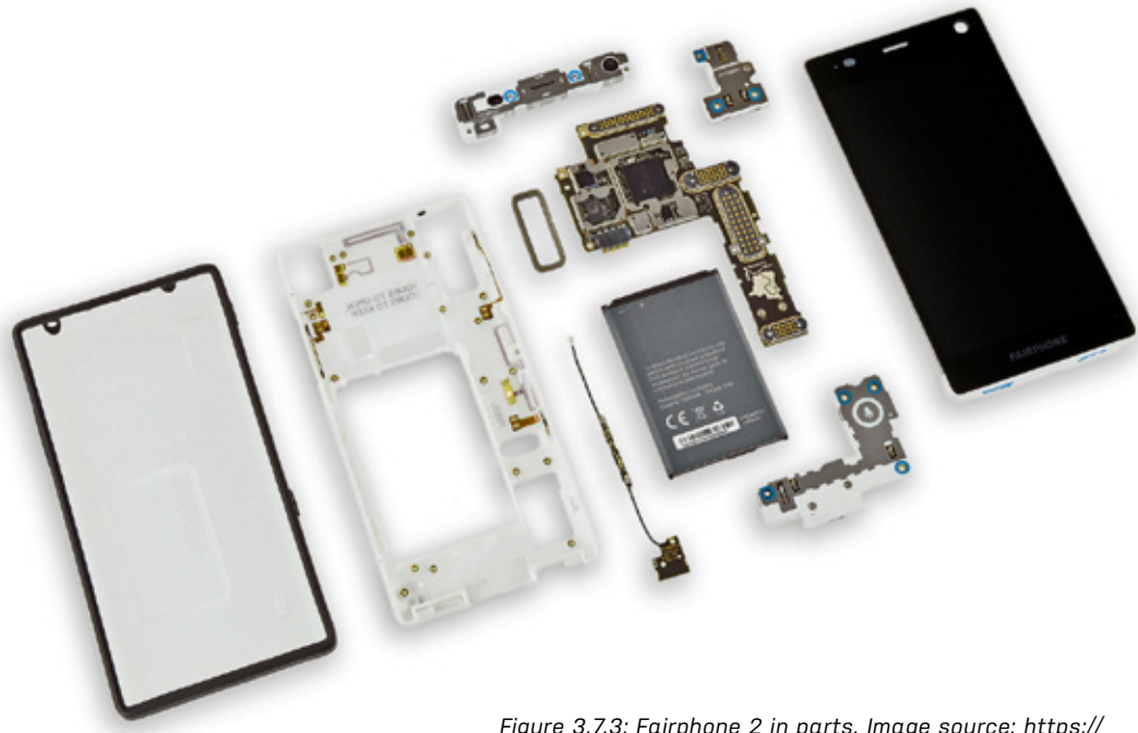
Figure 3.7.3: Fairphone 2 in parts. Image source: https://d3nevzfk7ii3be.cloudfront.net/igi/yXuyUATwQcmYlqID.huge
