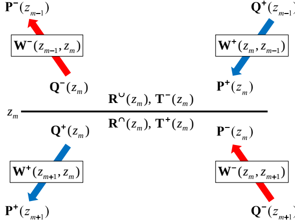
Figure B.1: The incoming and outgoing wavefields in the upward and downward directions, propagating between two depths levels, z_m and z_{m\pm 1} , as well as being reflected and transmitted at a depth level of z_m (after [1]).
