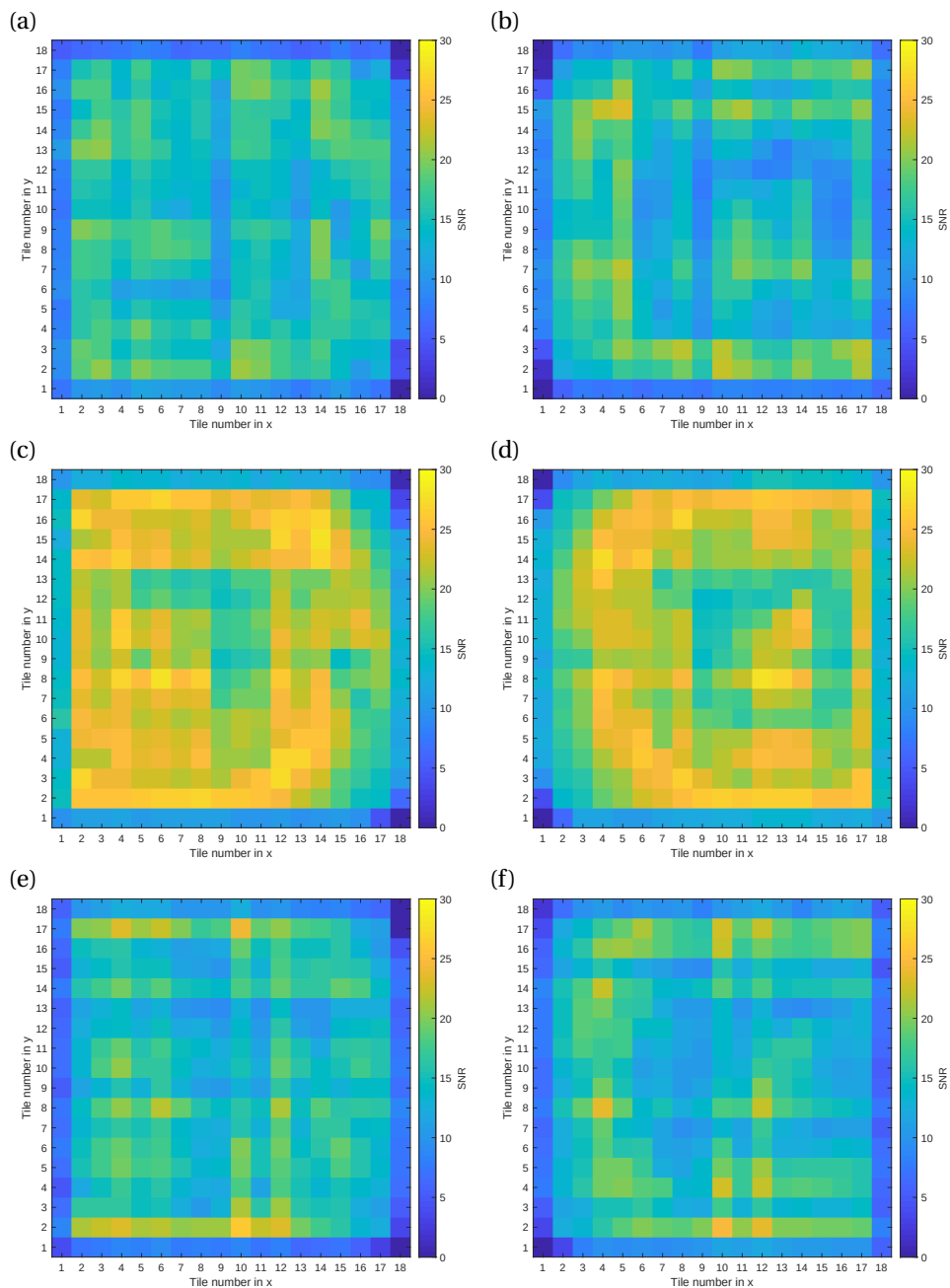
Figure 3.24: SNR values of OVIs. SNR values of \langle \mathcal{X}_i^k \rangle and \langle \mathcal{X}_j^k \rangle , (a)-(b) for the random designs, (c)-(d) for the quality designs and (e)-(f) for the economic design.
