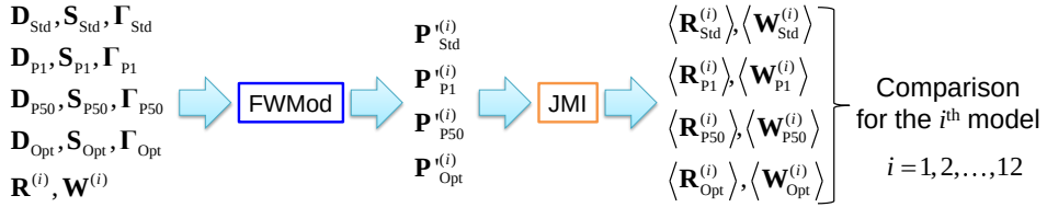
Figure 4.9: Analysis on the effect of uncertainty in prior subsurface information. (a) Various velocity perturbations applied to the subsurface model. (b) Procedure of the analysis for the i^{\text{th}} subsurface model. For subscripts in matrices, "Std", "P1", "P50" and "Opt" refer to the applied acquisition scenario.
