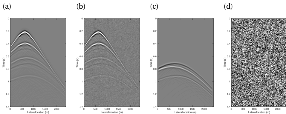
Figure 5.3: Unblended and well-sampled data. (a)-(b) Unblended and well-sampled shot records from the 1 st survey without and with incoherent noise. (c)-(d) Time-lapse responses between the 1 st and the 5 th surveys without and with incoherent noise, both of which are amplified by a factor of ten.
