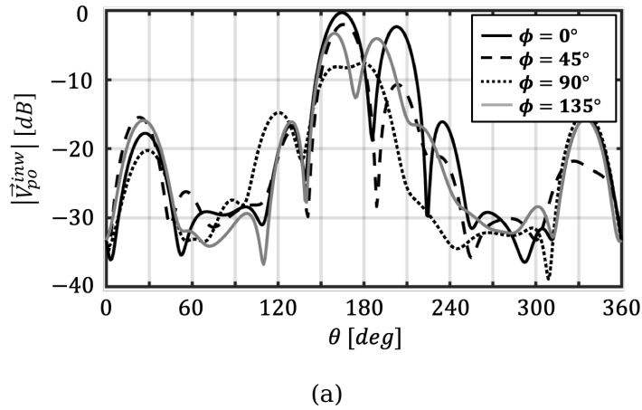
Figure 5.16: Normalised magnitude of the inward component of the observable field's pattern for four different \phi cuts in P2 at 115GHz (a) and 125GHz (b). Note that to highlight the beam splitting around \theta = 180^\circ the field is plotted for \theta = 0 \rightarrow 360^\circ
