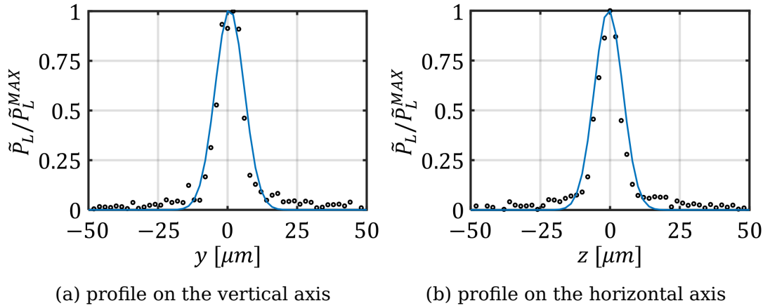
Figure 3.7: Profile of the focused optical beam obtained with the setup in Fig. 3.3 along the vertical (y) and horizontal (z) axis, respectively. The solid blue line is a Gaussian fit to verify the gaussicity of the focused beam. The -3dB diameter of the beam along the y axis is D_L^y = 10.2\mu m , on the z axis it is D_L^z = 9.5\mu m .
