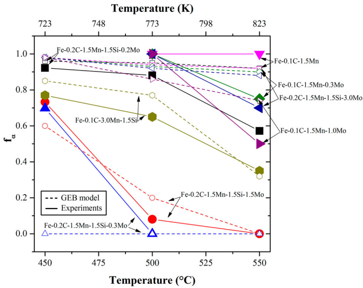
Figure 4. Comparison between predicted values of fraction of bainitic ferrite ( f_{\alpha} ) with the GEB model (shown with hollow symbols/dashed lines) and experimental reports (shown with solid symbols/solid lines) in Fe-0.1C-3.0Mn-1.5Si, Fe-0.1C-1.5Mn, Fe-0.1C-1.5Mn-0.3Mo, Fe-0.1C-1.5Mn-1Mo alloys Fe-0.2C-1.5Mn-1.5Si-xMo ( x = 0.2, 1.5, 3.0 mass%) [3,12,24].
