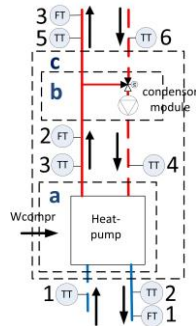
Fig. 2. Heat pump and condensor module
