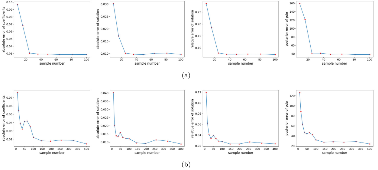
Fig. 6. Influences of the number of sampling points on performance, when the model is trained with L_{\phi_h} . (a) Curves of four performance indicators vs. S on human\_f_1 ; and (b) Curves of four performance indicators vs. s on flower\_f_1 . The abscissa of each picture is S , and the ordinate is the test indicator. The ordinates of each row from left to right are: absolute error of coefficients, absolute error of numerical solution, relative error of numerical solution, and posterior error of Poisson equation.
