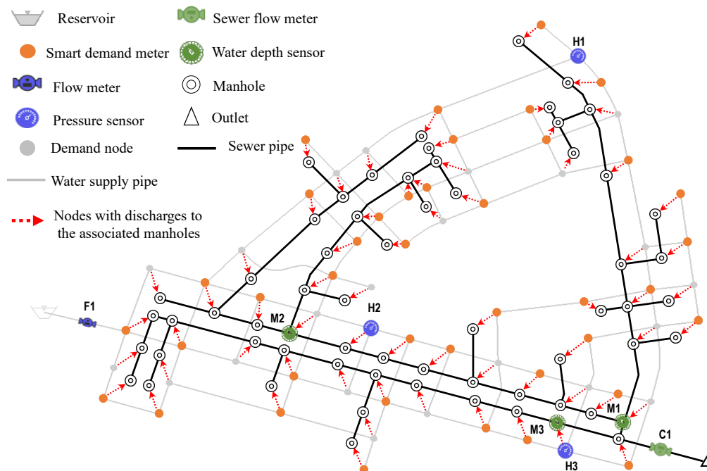
Fig. 4 The layout and sensor locations of the BKN case study and its corresponding WDS-BNK
