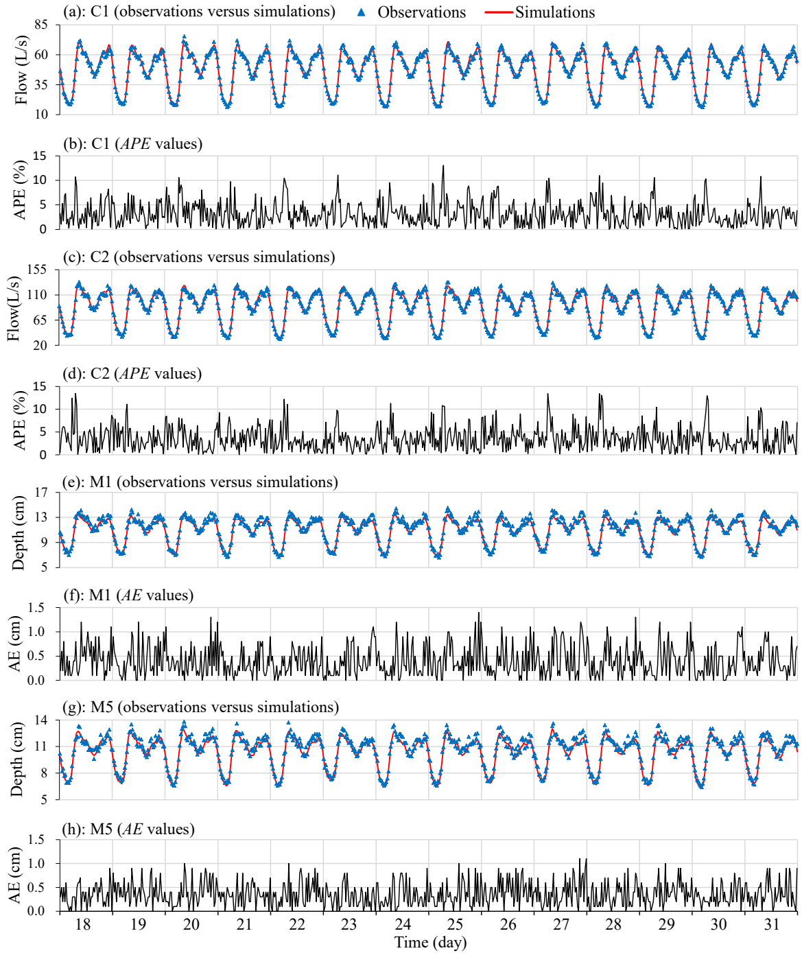
Fig. 12 Observations versus simulations, as well as the APEs or AEs for the four monitoring locations (shown in Fig. 5) within the validation period of the XZN case study
