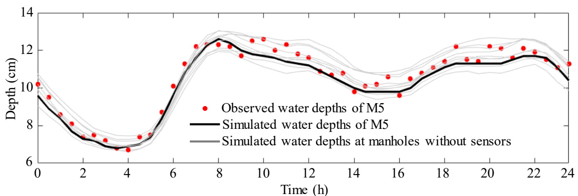
Fig. 13 Water depth simulations and observations of M5, as well as the water depth simulations of 10 manholes near M5 without sensors in the XZN case study in 18 th day within the validation period
