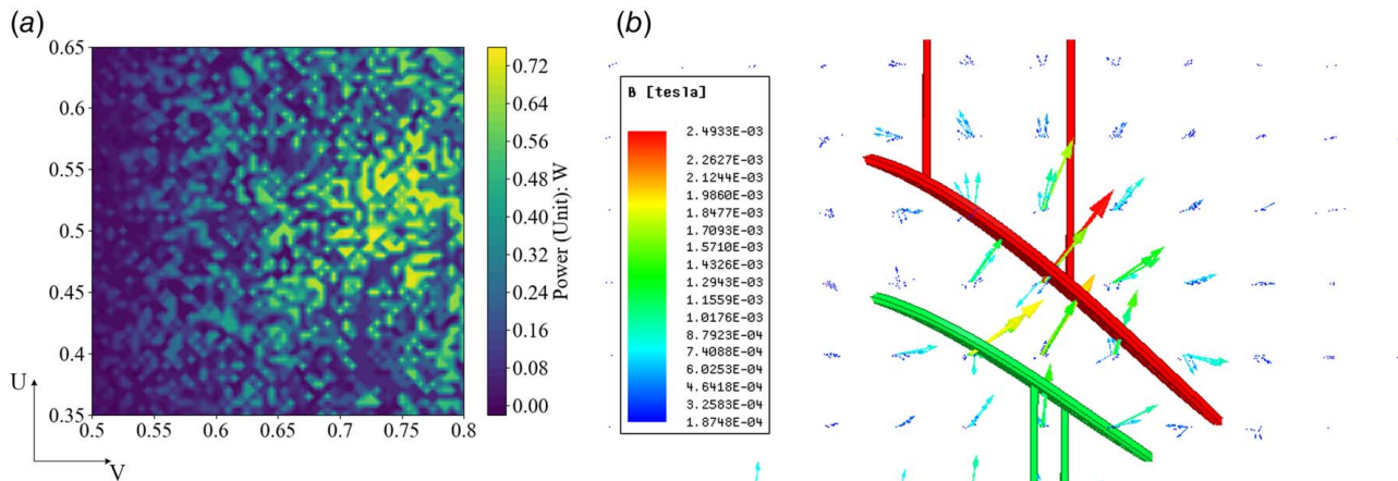
Fig. 7 Simulation results of a pair of optimized coils: (a) the relation between position and the power that can be transmitted and (b) B-field of the IPT system
