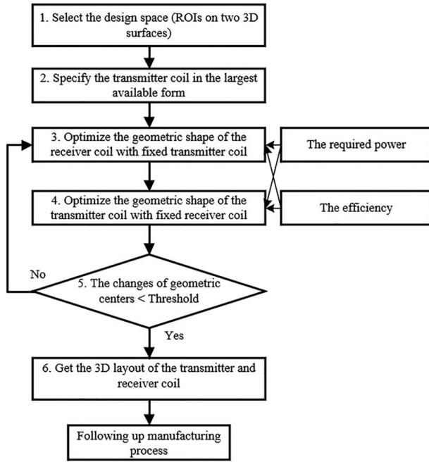
Fig. 1 The approach for designing 3D coils for IPT
