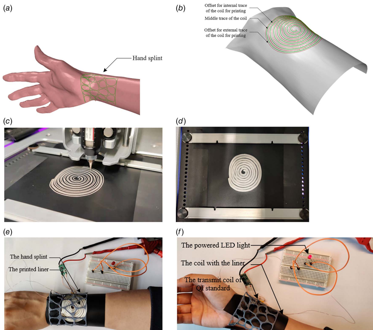
Fig. 11 A smart liner with an integrated IPT system for the hand splint: (a) the design of the hand splint, (b) the designed coil using the proposed approach, (c) the printing process, (d) the printed receiver coil, (e) the printed liner with the hand splint, and (f) power an LED light
