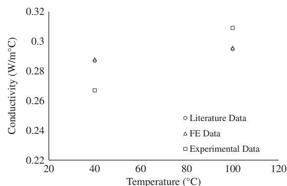
Figure 4. Thermal conductivity of glycerin.
