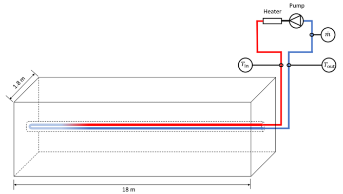
Fig. 2. A scheme of the prototype GSHP experiment, conducted by Beier et al. [26].
