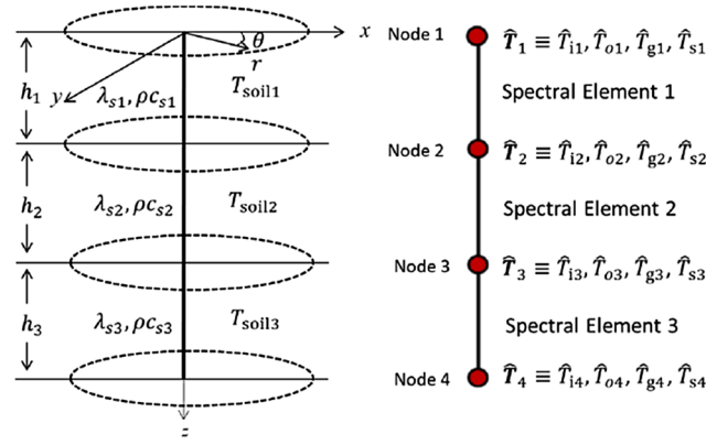
Fig. A2. A three-layer system and its spectral element discretization.
