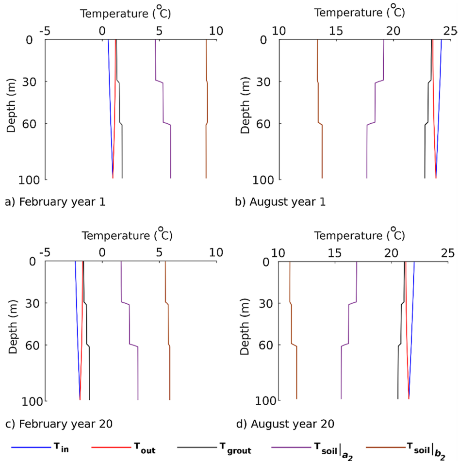
Fig. 10. Vertical temperature distributions in pipe-in, pipe-out, grout and soil for Case 2.
