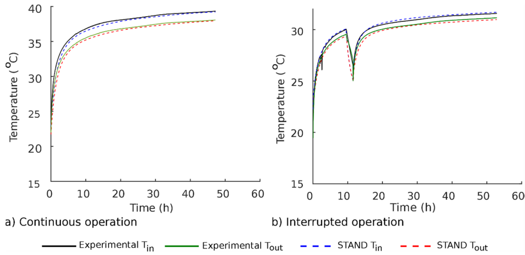
Fig. 4. Measured and computed temperature variations in time based on heat pump power.
