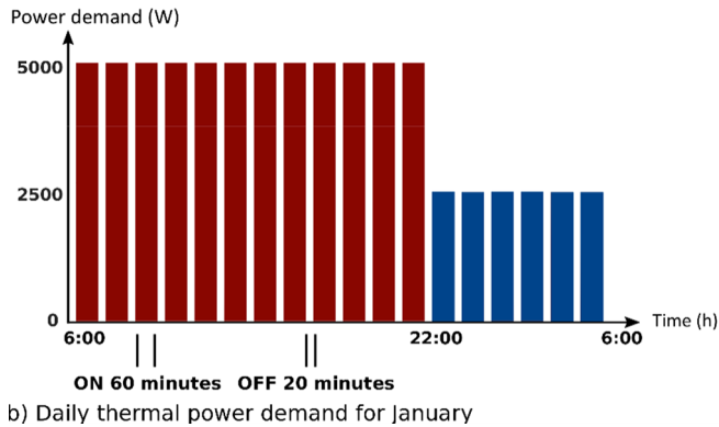
Fig. 7. Power demand from the ground.
