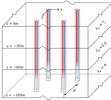
Fig. 5. A scheme of GSHP consisting of 4 BHEs embedded in 3 soil layers.
