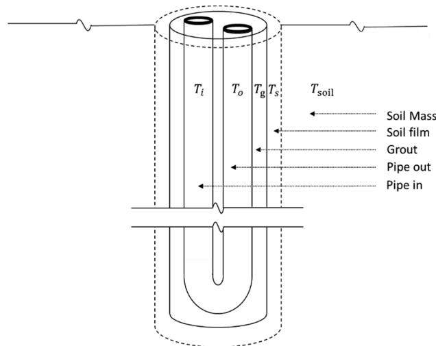
Fig. A1. A schematic representation of a single U-tube BHE and its surrounding soil mass.
