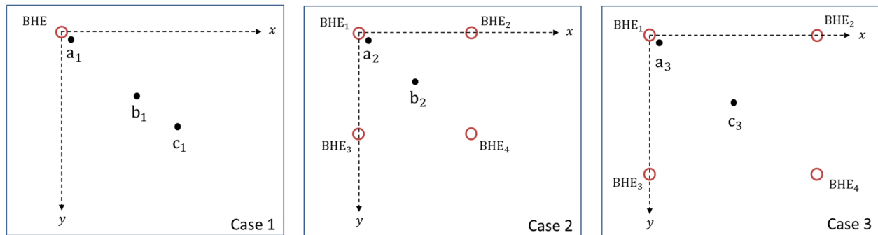
Fig. 6. Case 1: one active BHE; Case 2: four active BHEs, 5 \text{ m} \times 5 \text{ m} ; Case 3: four active BHEs, 8 \text{ m} \times 8 \text{ m} .
