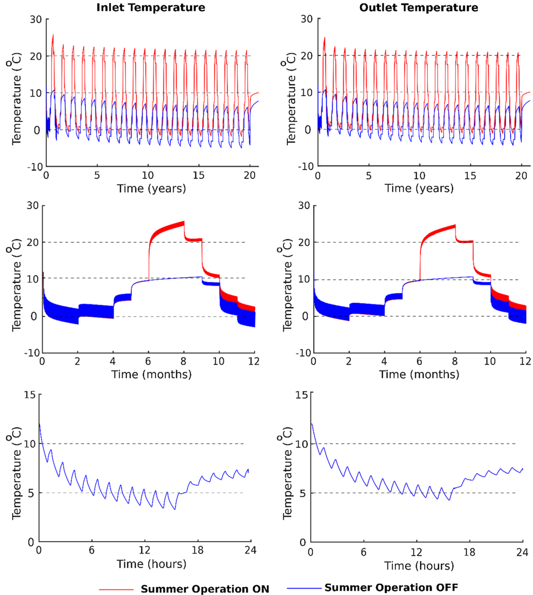
Fig. 9. Inlet and outlet temperatures for Case 2.
