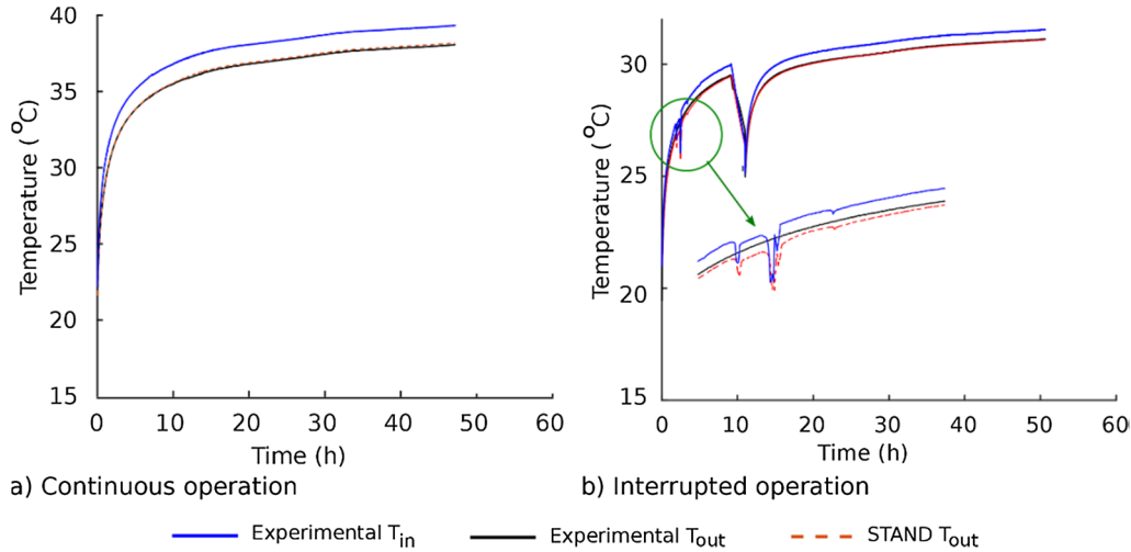
Fig. 3. Measured and computed temperature variations in time based on prescribed inlet temperature.
