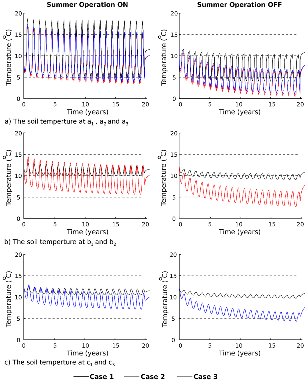
Fig. 8. Soil temperature at z = 100 m for Case1, Case 2 and Case 3.
