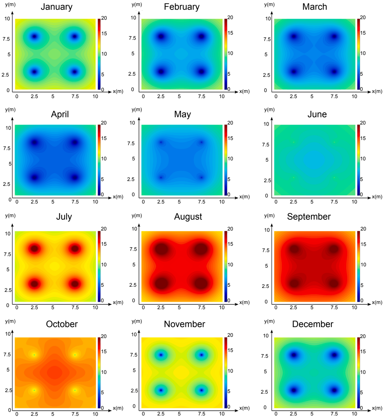
Fig. 11. Soil temperature snapshots at z = 100 m for Case 2.
