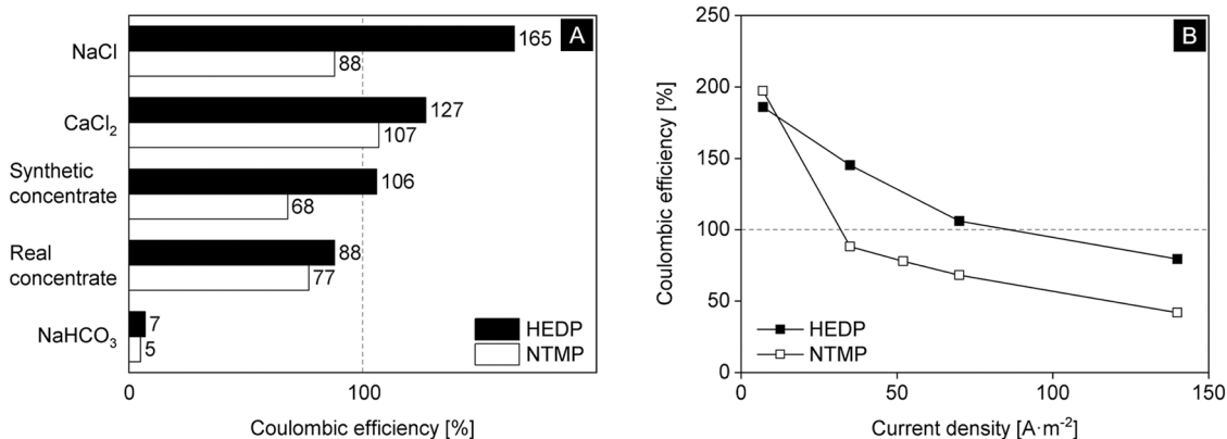
Fig. 12. (A) Coulombic efficiencies in different media for HEDP and NTMP phosphonates. (B) Coulombic efficiencies as a function of the current densities in synthetic concentrate. Current density: 70 \text{ A}\cdot\text{m}^{-2} , z = 2 in Faraday's Law.
