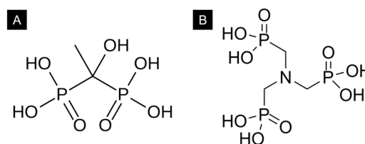
Fig. 1. : Molecular structures of the phosphonates (A) 1-hydroxyethylidene-1,1-diphosphonic acid (HEDP), and (B) Aminotris (methylenephosphonic acid) (NTMP or ATPM).
