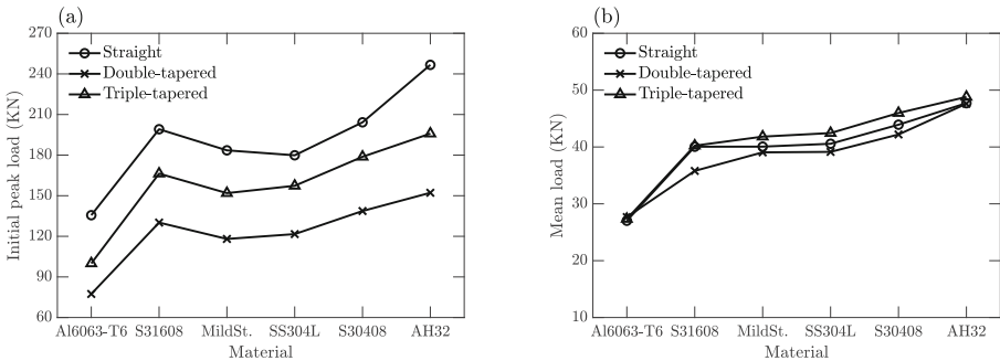
Fig. 5. (a) The variation of the initial peak load versus material, (b) the variation of the mean load versus material.
