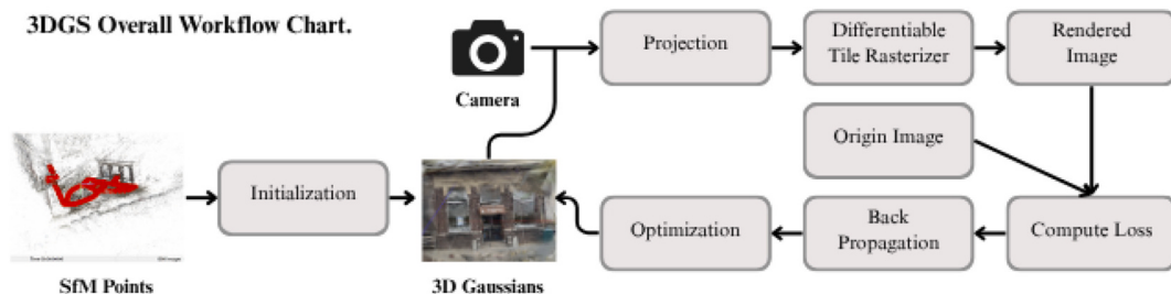
Fig. 1. Standard workflow for 3DGS [67].
