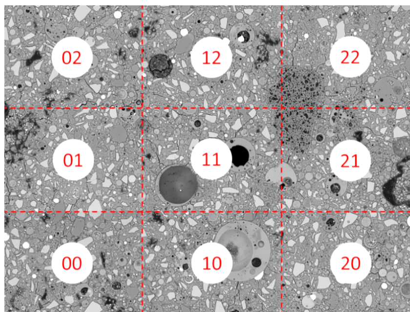
Figure 5. SEM-BSE image of the area of interest ( 3 \times 3 matrix (fields are labelled 00–22), with an individual SI field comprising of 512 \times 384 pixels) for paste microstructure characterization (sample is paste S50, unsealed cured for 28 days). All 9 fields of the area were analysed under the same analytical conditions. The total field width equals 750 microns.
