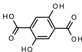
Scheme 1. The 2,5-dihydroxyterephthalic acid (H 4 DOBDC) used in the present study.
