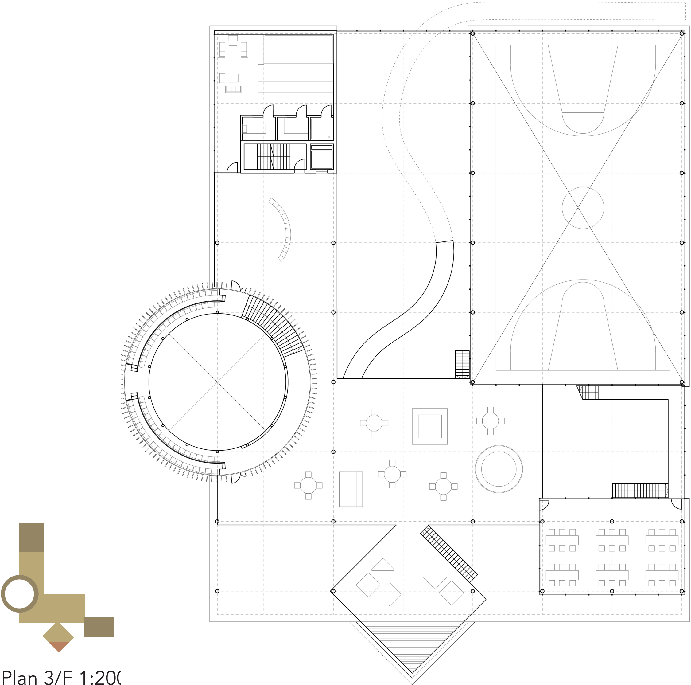
Plan 3/F 1:200
