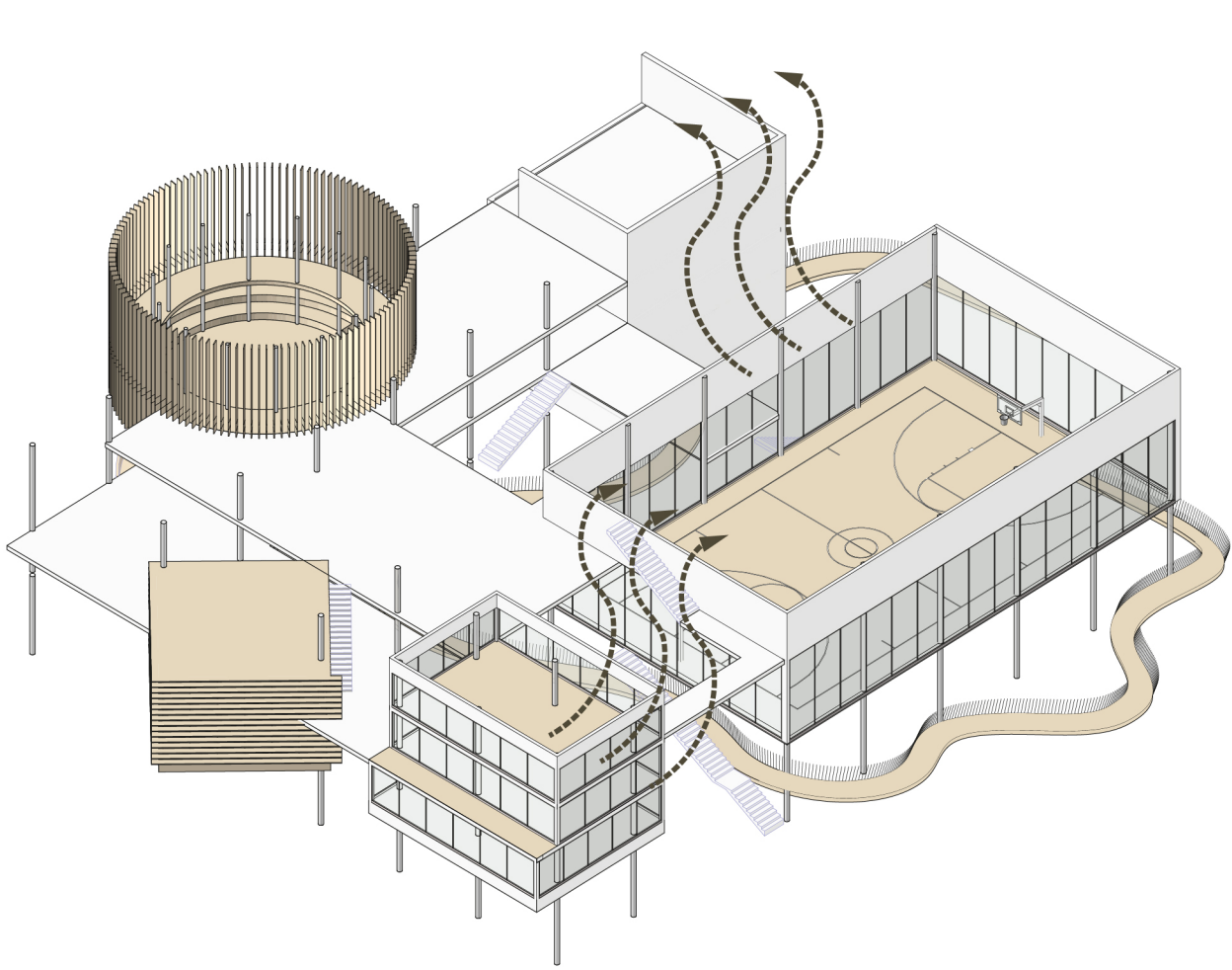
Natural ventilation
