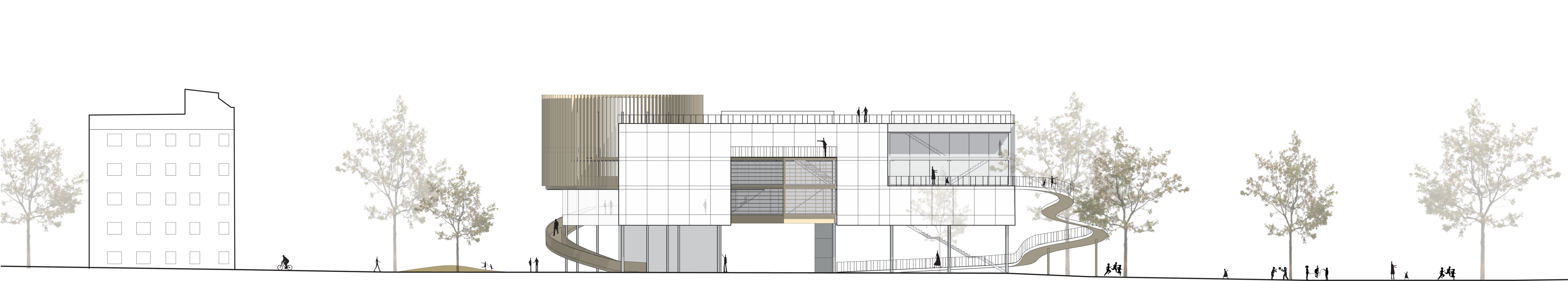
South elevation 1:200
