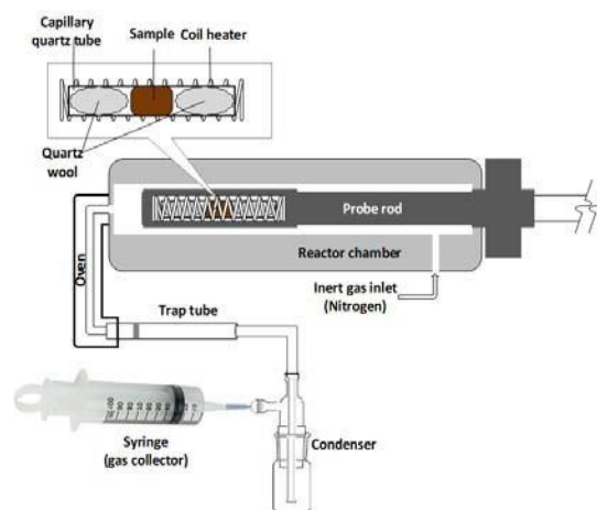
Figure 2: Schematic diagram of the pyroprobe reactor
