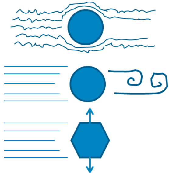
Figure 3: Top: turbulence; middle: vortex shedding; bottom: galloping.
