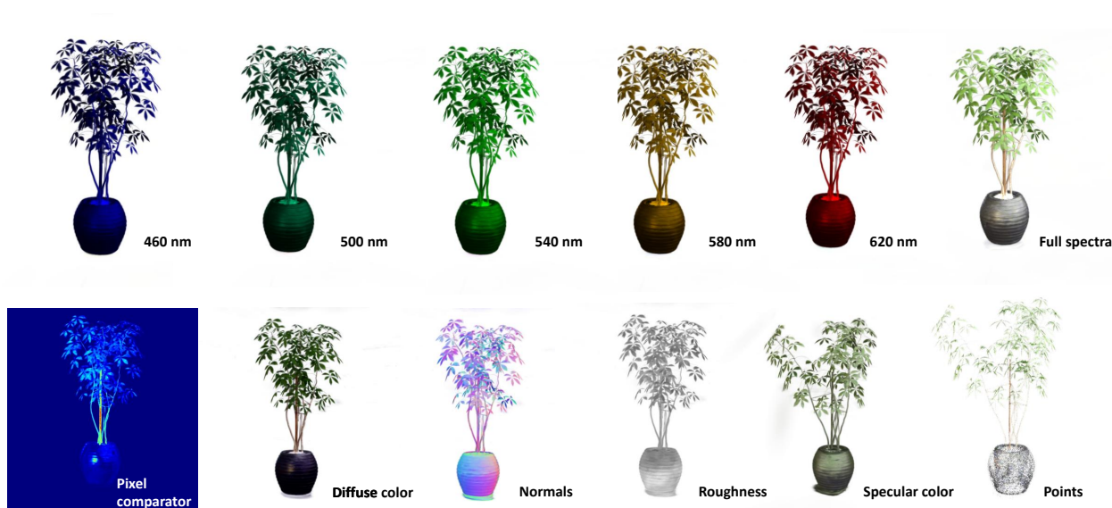
Figure 1: SpectralSplatsViewer: Visualization of Spectral renderings, reflectance parameters and pixel comparator mode of the Ficus scene
