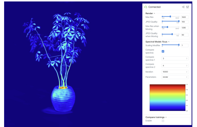
Figure 9: Spectra comparison mode (Ficus scene): Comparison of renderings at 580nm and 620nm
