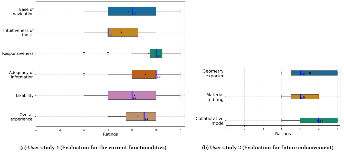
Figure 12: In the above figure, the statistical distribution of the ratings of the user-studies are presented. The inter-quartile range (IQR) is depicted as a colored box, with the median represented by a blue line inside the box and the mean indicated by an \times symbol. The whiskers of the box plot extend to 1.5 times the IQR. Any data points lying outside this range are shown as individual points, denoting them as outliers.
