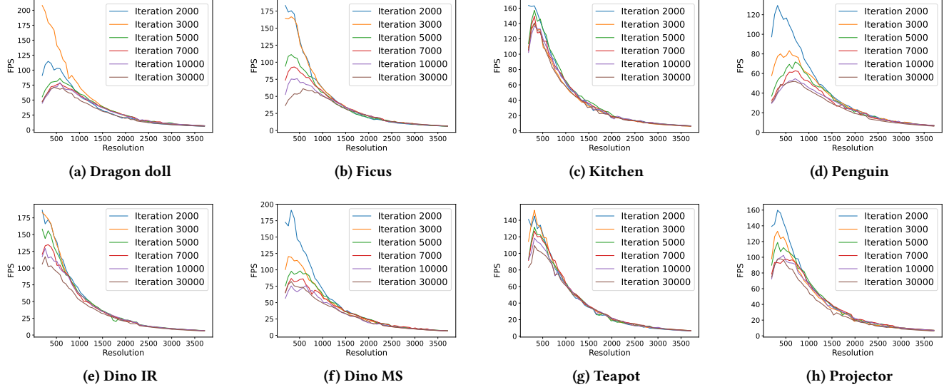
Figure 7: Frames per second (FPS) of scenes at different resolutions and training iterations (i.e having different number of Gaussians).
