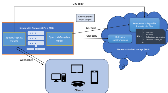
Figure 3: SpectralSplats Viewer: Architecture
