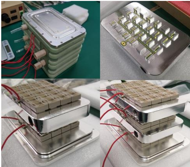
Figure 5. The IGBT press-pack module after packaging and its internal structures.
