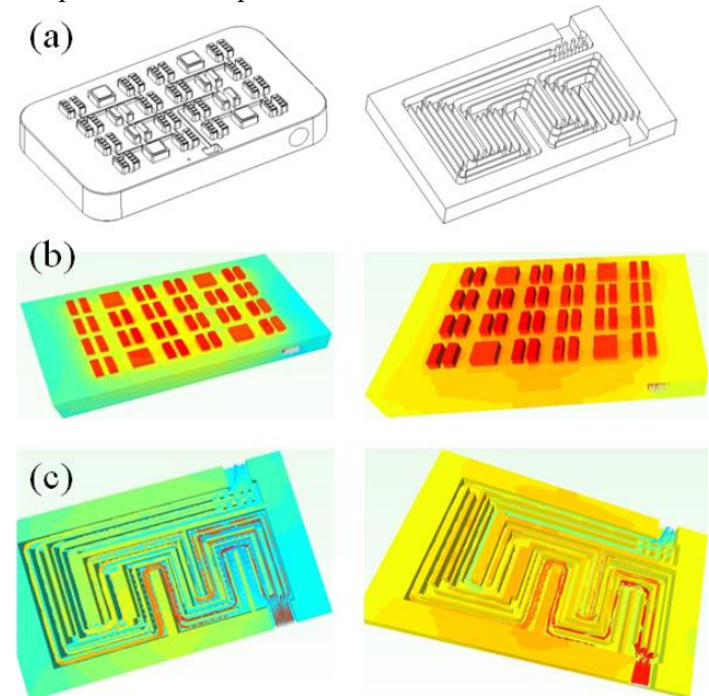
Figure 3. (a) The cooling baseplate and its internal channel. The thermal distribution with the inlet temperature of (b) 30 °C and (c) 54 °C.
