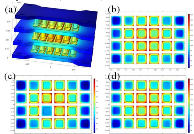
Figure 4. The thermal distribution of (a) the proposed IGBT module, (b) first subunit, (c) second subunit, and (d) third subunit.
