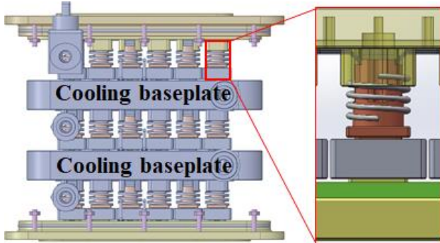
Figure 2. Cooling baseplate and press-pack structure.
