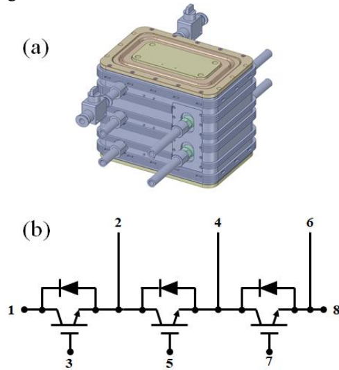
Figure 1. (a) Packaging scheme and (b) circuit topology of 1kA/10 kV IGBT press-pack module.
