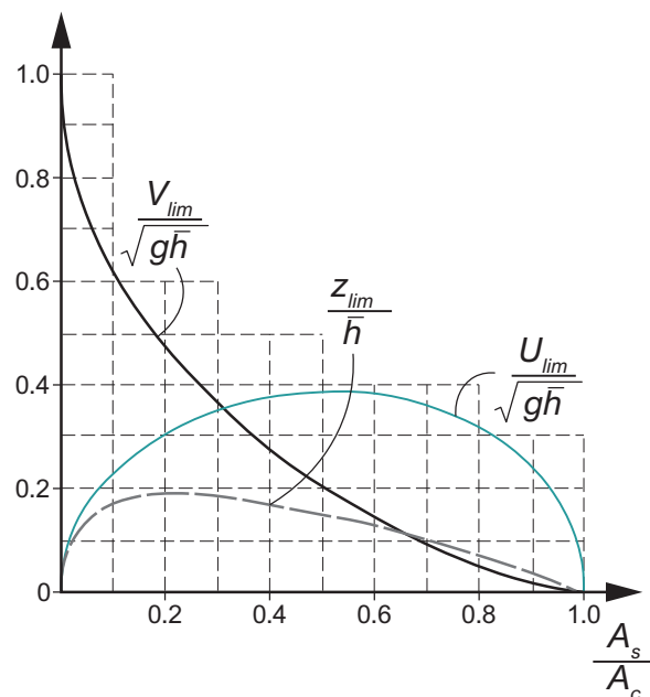
Figure 4.4: Limit values according to Schijf's theory (by TU Delft – Ports and Waterways is licenced under CC BY-NC-SA 4.0).
