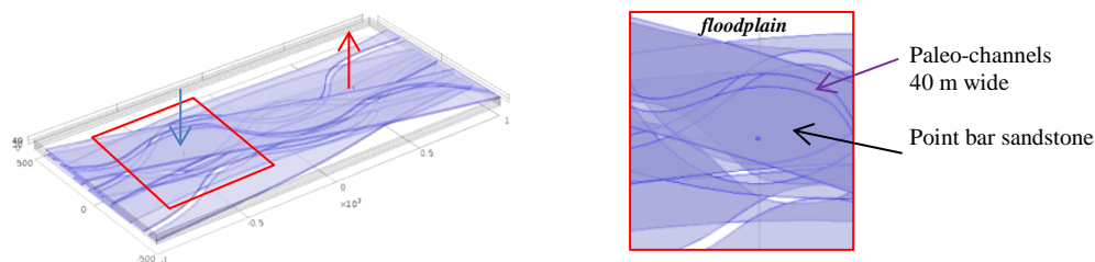
Figure 9: Left) Reservoir model level 4 overview. Right) Close-up of the topview of the geological features in the model.
