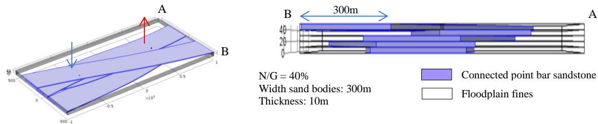
Figure 8: Left) An overview of geological features in the model. Right) A cross-section A-B with a side view of the model.
