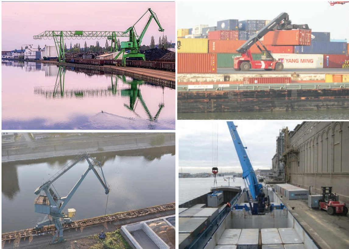
Figure 5.36: Examples of (un)loading facilities; upper left: gantry crane by Jürgen Striewski is licenced under CC BY-SA 4.0, upper right: reach stacker by Lundex is licenced under CC BY-SA 2.5, lower left: quay mounted crane by Atamari is licenced under CC BY-SA 3.0, lower right: vessel mounted crane (from www.slideshare.net , “Crane Barges”, Copyright by Mercurius Shipping Group).
