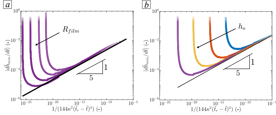
Figure 4.7 Dimensionless thinning rate as a function of the rescaled time axis (based on Eq. 4.14) illustrating late stage film dynamics for a fixed initial film thickness of h_o = 2000 nm and different R_{film} = 50 \mu\text{m} , 100 \mu\text{m} , 200 \mu\text{m} and 400 \mu\text{m} in (a); and for a fixed film radius of R_{film} = 100 \mu\text{m} and different h_o = 300 nm, 500 nm, 1000 nm and 2000 nm in (b). The black solid lines correspond to Eq. 4.14.
