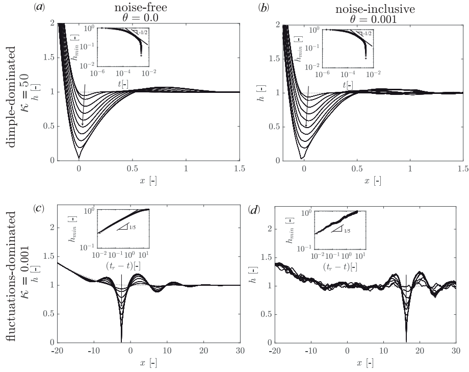
Figure 3.3 Comparison between films with high ( \kappa \gg \kappa_{lr} , dimple-dominated) and low ( \kappa \ll \kappa_{lr} , fluctuations-dominated) curvature, without ( \theta = 0 ) and with realistic ( \theta = 0.001 ) noise. (a) Evolution of film heights in the dimple region for \kappa = 50 for a deterministic simulation, at various dimensionless times t = (0.01, 0.03, 0.08, 0.16, 0.28, 0.45, 0.75, 1.3, 2.1, 2.5) \cdot 10^{-3} (also reported in 14 ); (b) Evolution of film heights in the dimple region for \kappa = 50 for a single realization of a stochastic simulation, at various dimensionless times t = (0.01, 0.02, 0.07, 0.14, 0.28, 0.5, 0.87, 1.4, 2.0, 2.3) \cdot 10^{-3} . (c) Evolution of film heights for \kappa = 0.001 for deterministic simulations, at various dimensionless times, t = (7, 10, 13.6, 14.7, 15.2, 15.5, 15.55, 15.58, 15.6) ; (d) Evolution of film heights for \kappa = 0.001 for a single realization of a stochastic simulation at various dimensionless times, t = (1.6, 3, 5.04, 5.7, 6.16, 6.27, 6.37) . The insets in (a-d) show the corresponding time evolutions of the minimum film height.
