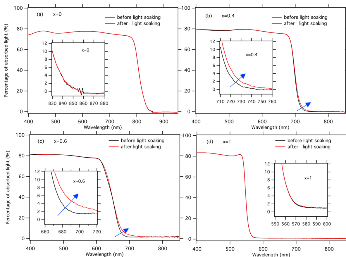
Figure 1. Absorbance spectra before and after LS in N_2 for (FA_{0.79}MA_{0.15}Cs_{0.06})Pb(I_{1-x}Br_x)_3 with x = 0, 0.4, 0.6 , and 1 . The blue arrows indicate the shift due to the LS. For comparison, the effect of LS on MAPb(I_{0.6}Br_{0.4})_3 is shown in Figure S3b. The insets are magnifications to show the subtle shift due to the LS.
