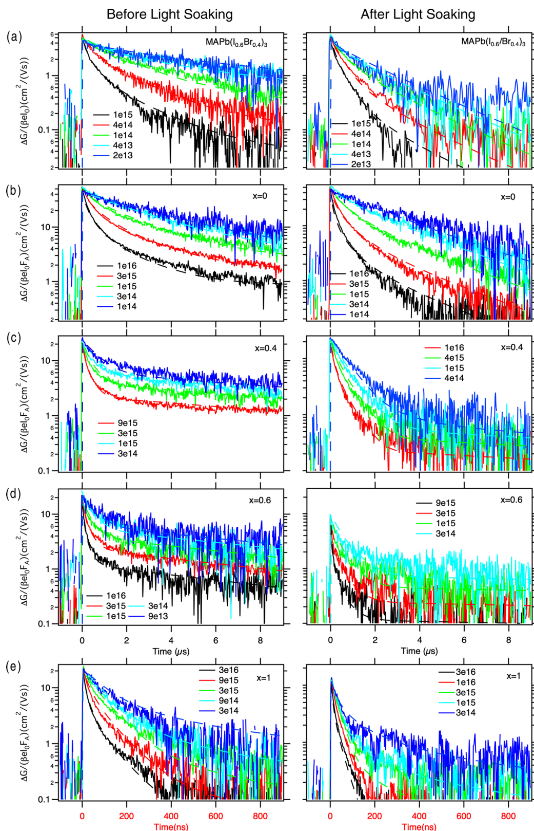
Figure 3. TRMC traces of MAPb(I 0.6 Br 0.4 ) 3 (a) and (FA 0.79 MA 0.15 Cs 0.06 )Pb(I 1-x Br x ) 3 for (b) x = 0 , (c) 0.4, (d) 0.6, and (e) 1 before (left panels) and after (right) LS. The analogues x = 0.2 and 0.8 are shown for comparison in Figure S5. Solid lines are the experimental traces, and dashed lines are the results of the fits. Note that panel (e) has a different time scale of 1 \mu\text{s} . The samples were all excited by laser pulses at 500 nm with excitation intensities leading to charge carrier densities ranging from 10 14 to 10 16 cm -3 , and specific densities are given in the annotations.
