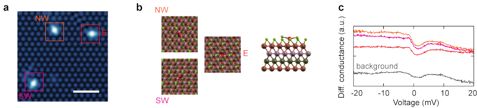
Figure 7.3: First excited state binding configuration for Co adatom on 1/3ML \sqrt{3}R30^\circ Cl-reconstructed Cu(111) – “arrow” (A). a STM topography of three Co adatoms in a linear geometry configuration. Each Co adatom connects two Cl atoms along three 120^\circ -split directions, forming arrow-like features. The only three possible pointing directions for arrow-like adatoms – North-West (NW), East (E) and South-West (SW) – are shown here. Imaging setpoint: I = 100 pA, V = 20 mV, T = 1.17 K; scale bar 2 nm. b Corresponding binding sites as obtained from DFT. Areas correspond to the squares encircling adatoms in topography in (a). Co adatom has two nearest Cl neighbours and occupies the hollow hcp site in-between resulting in its non-equidistant placement between the two Cl atoms and therefore unique pointing vector in all three directions. To the far right a side view for this binding configuration showing Co adatom with a bonding asymmetry along the Cl-Co-Cl direction appearing slightly lower compared to the Cl atoms it binds to. Color code for DFT results as in Figs. 4.9b and 7.1a. c Corresponding IETS spectra taken on instances of these three arrow types with the same STM tip used for spectroscopy on RT adatoms from Fig. 7.1. Notice no difference in spectroscopy for the three pointing directions. Spectra offset for clarity. IETS settings: V_{\text{mod}} = 100 \mu V, T = 1.17 K.
