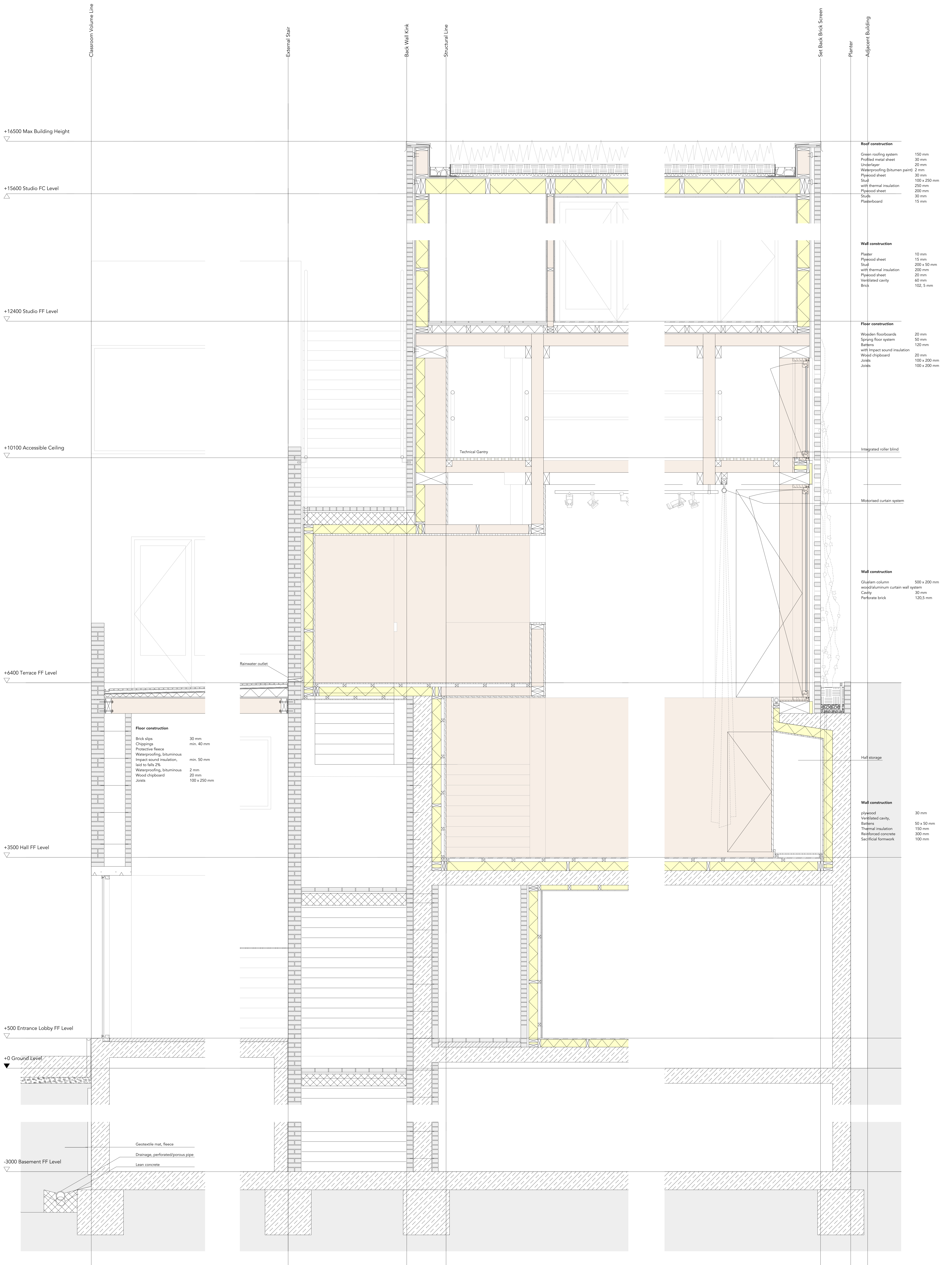
Detail Section 1:20
