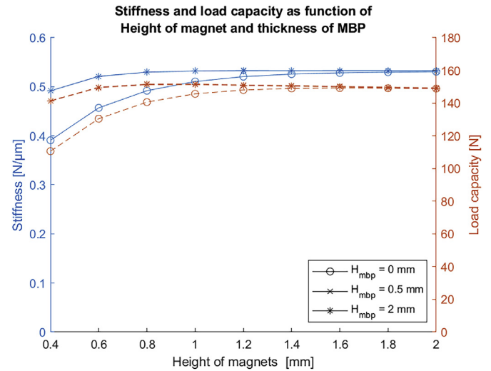
Fig. 6. Stiffness and load capacity as a function of height of magnet for different thicknesses of the metal bottom plate. For up-down magnetization configuration. The lines for 0.5 mm and 2 mm bottom plate thickness coincide.
