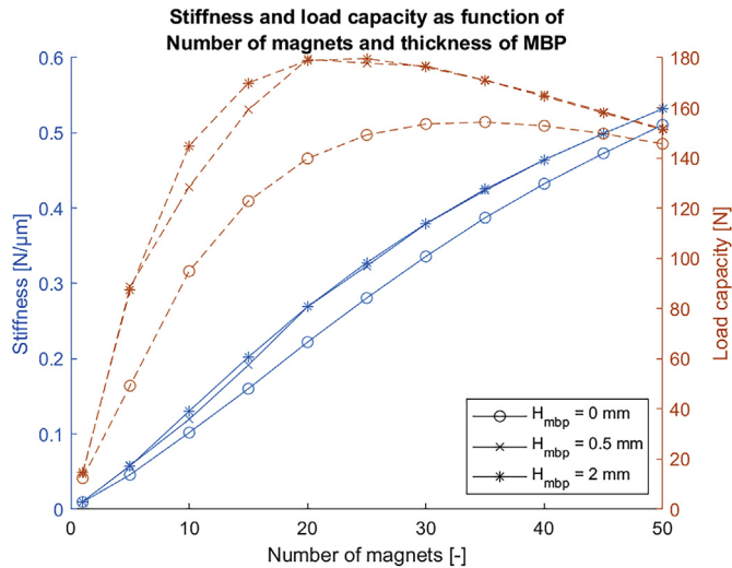
Fig. 4. Stiffness and load capacity as a function of the number of magnets for different thicknesses of the metal bottom plate. For up-down magnetization configuration.
