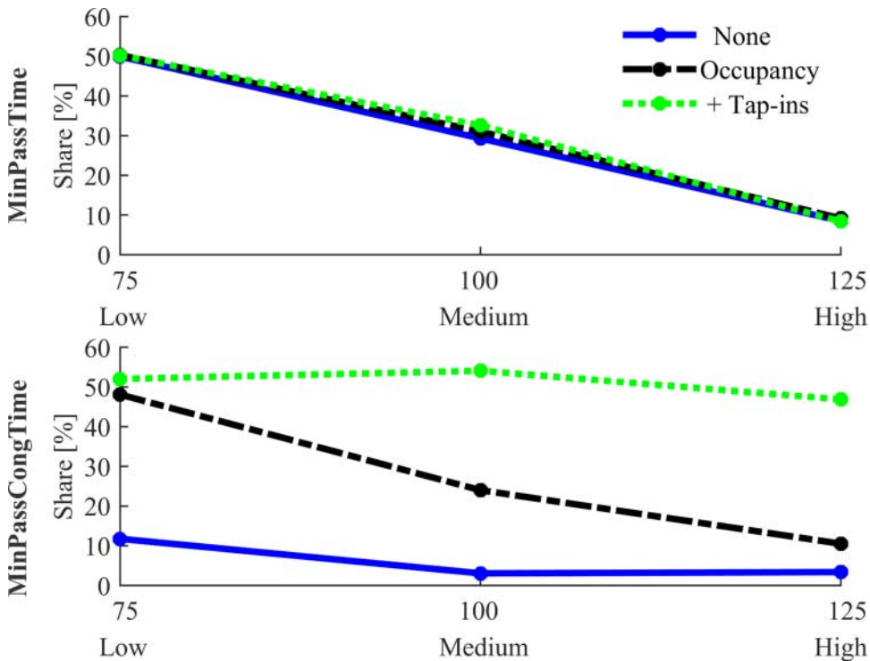
Figure 6. Share of synchronization control decisions per demand scenario (base case level = 100) and controller.
