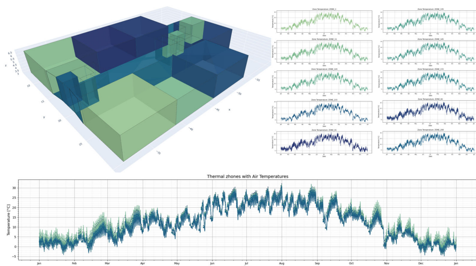
Figure 17. Topologic Solid Model ( CellComplex ) with proof-of-concept simulations temperatures.
