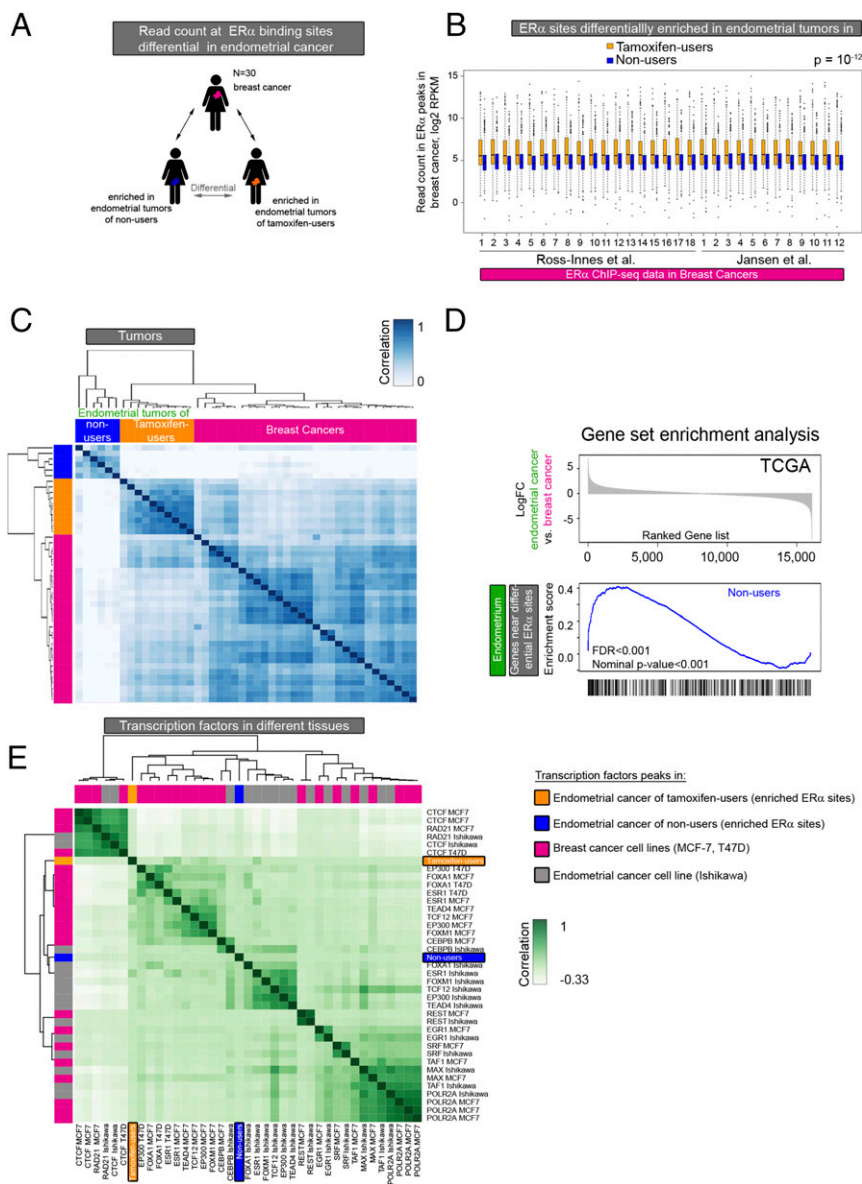
Fig. 4. Comparative analysis of ER \alpha -binding sites in endometrial and breast tumor tissue. (A) Analysis set-up. ER \alpha binding in breast cancer at the differential sites in the two endometrial cancer groups was evaluated. (B) Boxplot showing the normalized ER \alpha ChIP-seq read count in breast cancers at the ER \alpha -binding sites differentially enriched in endometrial tumors from tamoxifen users (orange boxplots) and nonusers (blue boxplots). The P value of the paired t test is P = 10^{-12} . (C) Heatmap visualization of the correlation matrix based on ER \alpha ChIP-seq read count at differential ER \alpha -binding sites in endometrial tumors of tamoxifen users (orange) and nonusers (blue) and in breast tumors (pink). (D) GSEA based on differential gene expression in endometrial and breast cancers from the TCGA pan-cancer project. (Upper) Ranked log-fold change in gene expression in endometrial cancer vs. breast cancer. (Lower) Enrichment scores vs. gene rank in the significantly enriched gene set: genes proximal to the binding sites enriched in tumors of nonusers. (E) Hierarchical clustering of the correlation between transcription factor genomic occupancy (peaks) from publicly available ChIP-seq data in the breast cancer cell lines MCF-7 and T47D (pink), the endometrial cancer cell line Ishikawa (gray), and the ER \alpha sites enriched in endometrial tumors from tamoxifen users (orange) and nonusers (blue).
