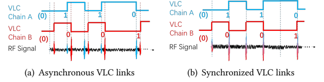
Figure 2: Received side-channel signal from two VLC chains.
