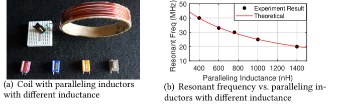
Figure 6: Experiment with paralleling inductors.
