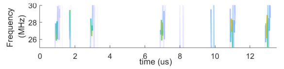
(b) Signals after Hilbert-Huang transform
