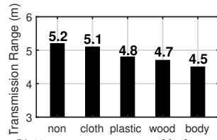
(b) Transmission range vs. blockages
