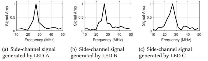
Figure 15: The frequencies of the side-channel signals generated by homogeneous LEDs.
