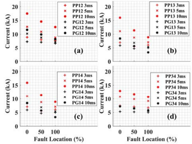
Fig. 5 Results of the possible pole to pole and pole to ground faults with different operation time in test topology; (a) fault in cable 12 (b) fault in cable 13 (c) fault in cable 14 and (d) fault in cable 34
