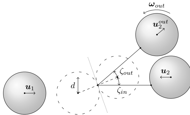
Figure 7.12: An oblique collision between two particles.
