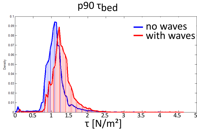
Figure 5.18: Spatial distribution (in % of the area) of the total bed shear stress that is exceeded 10% of the time.
