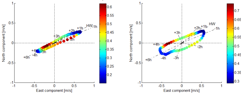
Figure 2.21: Tidal ellipse with the color scale indicating \widetilde{R}_0 for Blankenberge (left panel) and MOW1 (right) (De Maerschalck et al., 2020).
