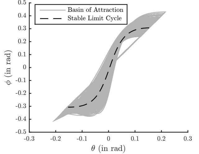
Fig. 2. Joint trajectories of the basin of attraction for the simple walking model with \gamma = 0.004 rad, m_h = 1 kg, m_f = 0.001 kg, L = 1 m, and g = 10 m/s 2
