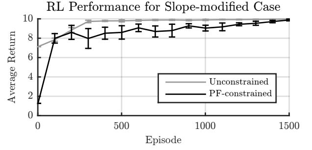
Fig. 9. Mean performance of the RL for the Unconstrained and PF-constrained policies for the Slope-modified case averaged over 10 runs with the error bars indicating the standard deviation. For both policies the exploration variance decreased linearly from 1e-6 to 1e-11 throughout the episodes.
