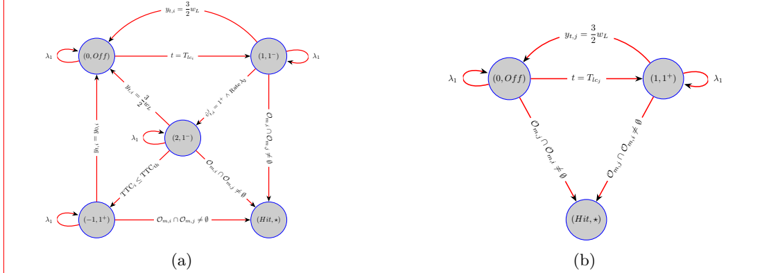
Figure 4: Transition graphs of the GSHS models for AVs i = ER and j = EL are shown in Figures (a) and (b), respectively. In these diagrams, w_L denotes the lane width, while T_{lc_i} and T_{lc_j} represent the time instants at which AVs i and j initiate their lane-change decisions. The inferred intent \hat{v}_{t,i}^j is derived from the SA's discrete state.
