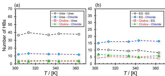
Figure 10. Number of hydrogen bonds as a function of temperature for the (a) reline–water mixture with a mass fraction of water of 40% and the (b) ethaline–water mixture with a mass fraction of water of 40%. Each simulation of reline contains 50 choline chloride molecules and 100 urea molecules. Each simulation of ethaline contains 50 choline chloride molecules and 100 ethylene glycol molecules.
