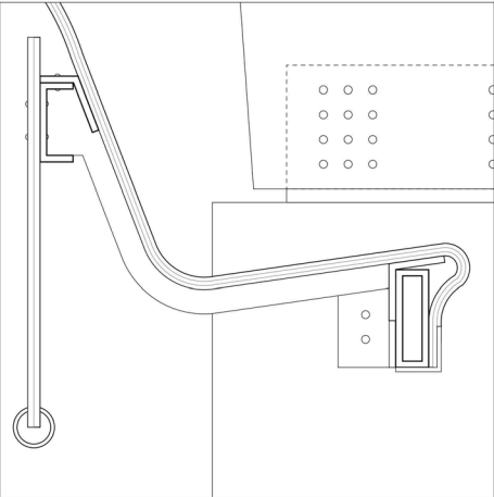
1 : 5 Bench Molded plywood 18 mm
