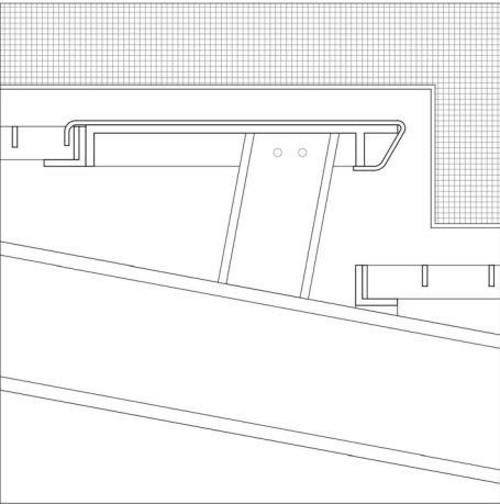
1 : 5 Handrail Molded plywood 18 mm Step Perforated stainless steel nosing 5 mm
