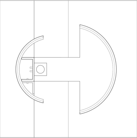
1 : 5 Lamp shade Molded plywood
