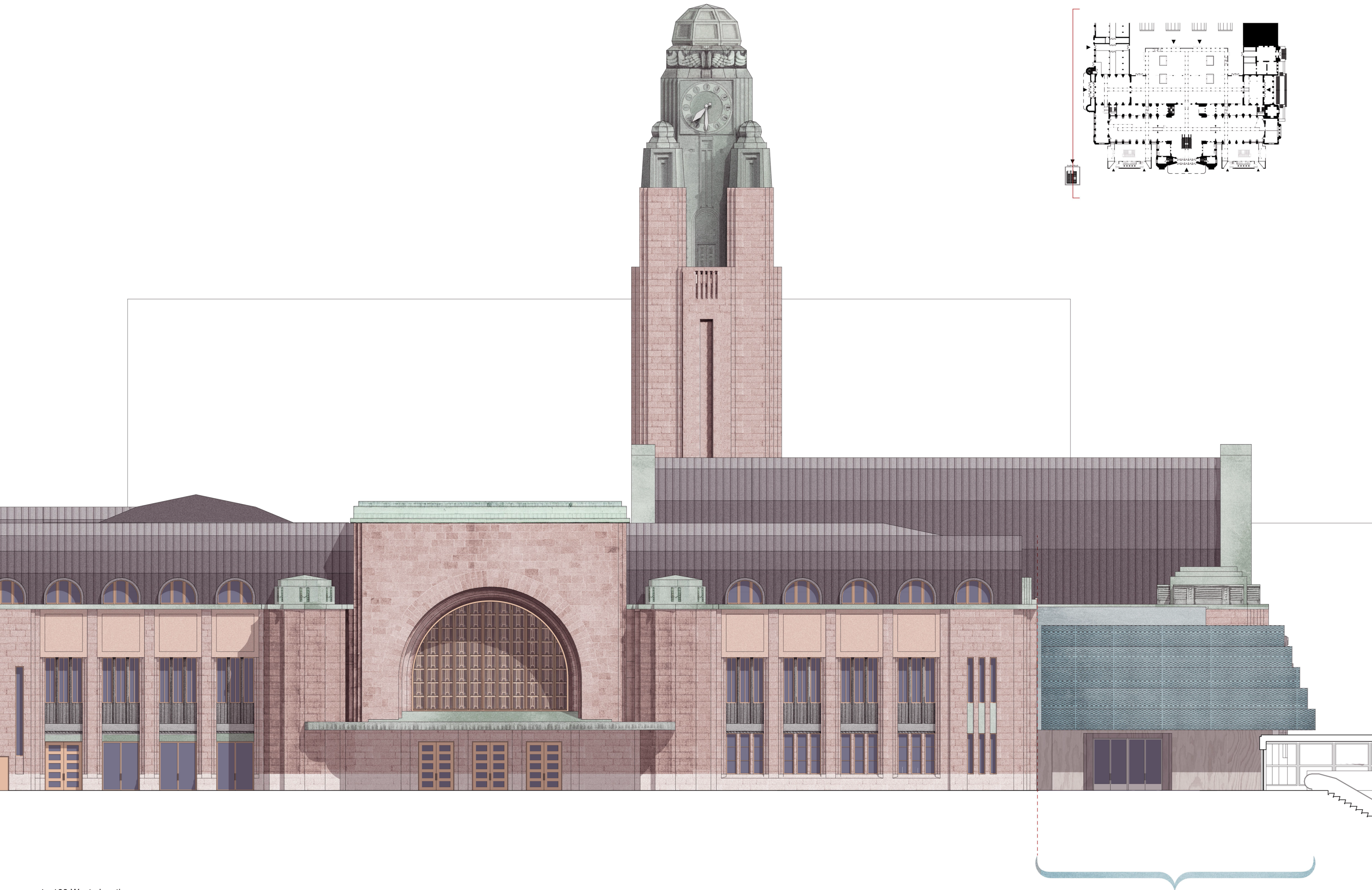
1 : 100 West elevation
