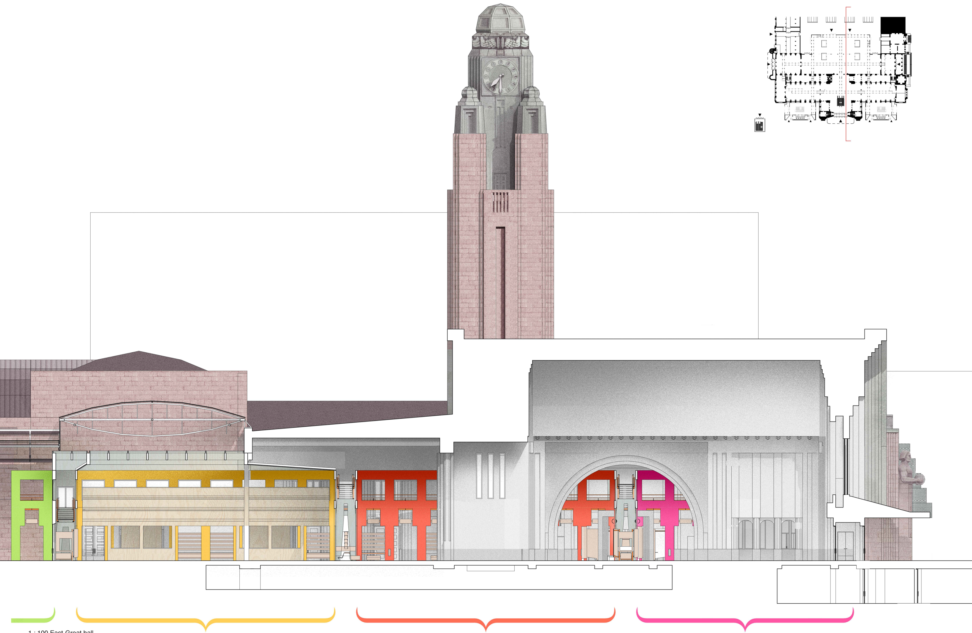
1 : 100 East-Great hall
