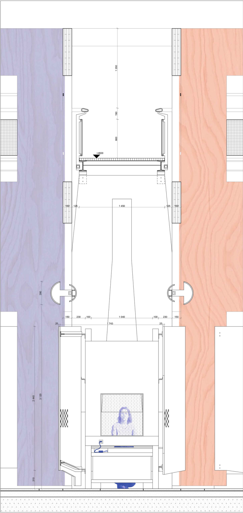
1. Wall panel Laminated solid wood wall element 150 mm Outer surface: water-based semi-transparent matte colour finish Both surfaces: Transparent matte top coat Connections with internal knife plates 2. Elevated walkway Grated steel floor panel 40 mm Steel beam 178x102x19 mm Steel connection with internal knife plate CLT cross beam 400 mm All steel surfaces with orange coating
