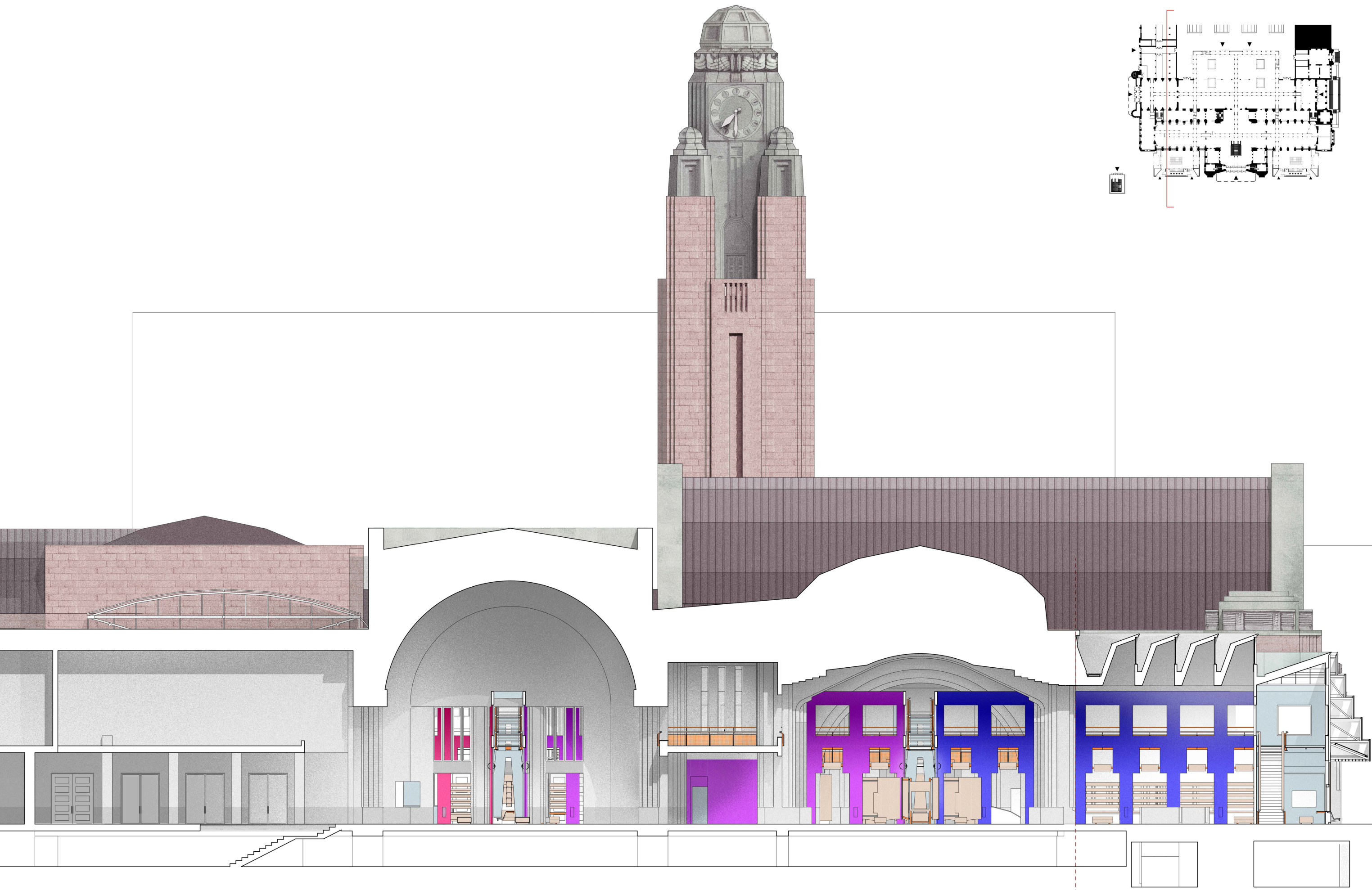
1 : 100 West-West vestibule
