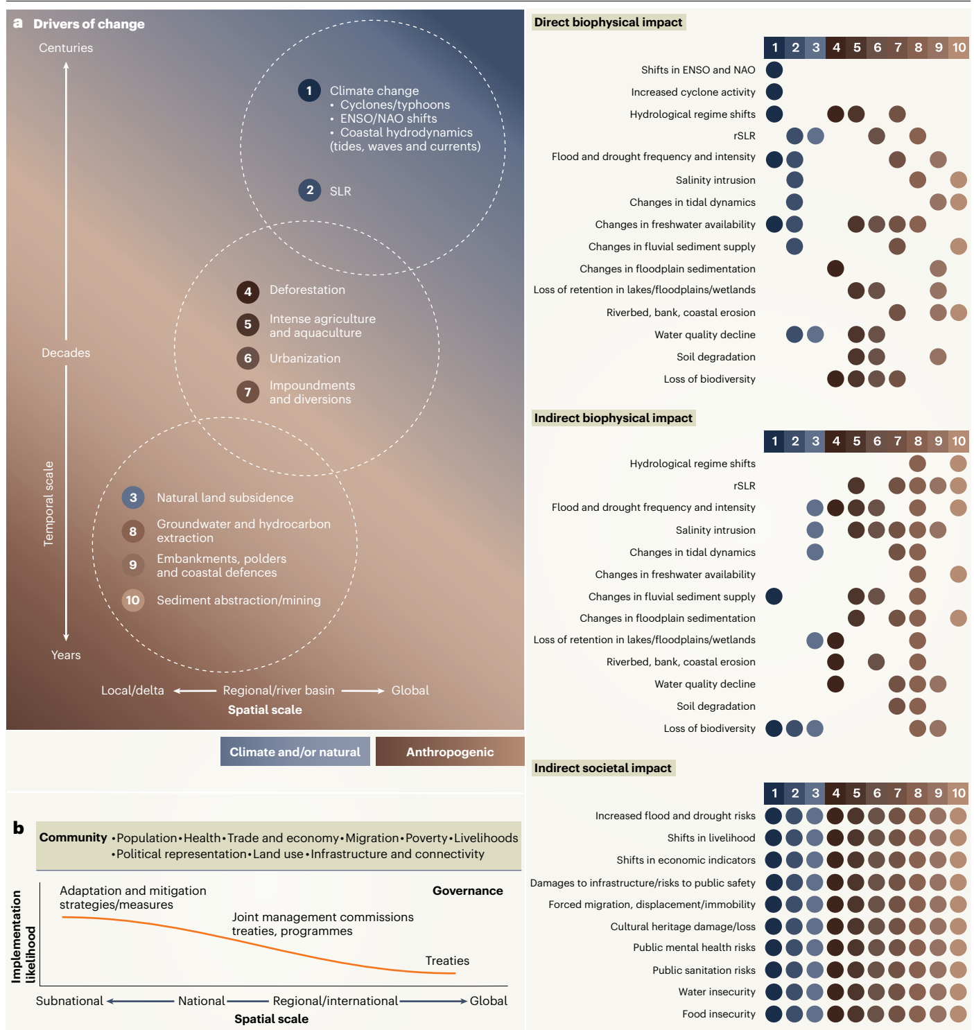
Fig. 2 | A conceptual framework to support decision-makers in addressing biophysical and societal challenges in deltas. a. Key drivers of change in river deltas divided into climate/natural and anthropogenic processes at various spatial and temporal scales, and their predominant direct and indirect impacts on the biophysical and socioeconomic systems (tables on the right). b. The drivers in a are influenced by and shape the community and the governance
