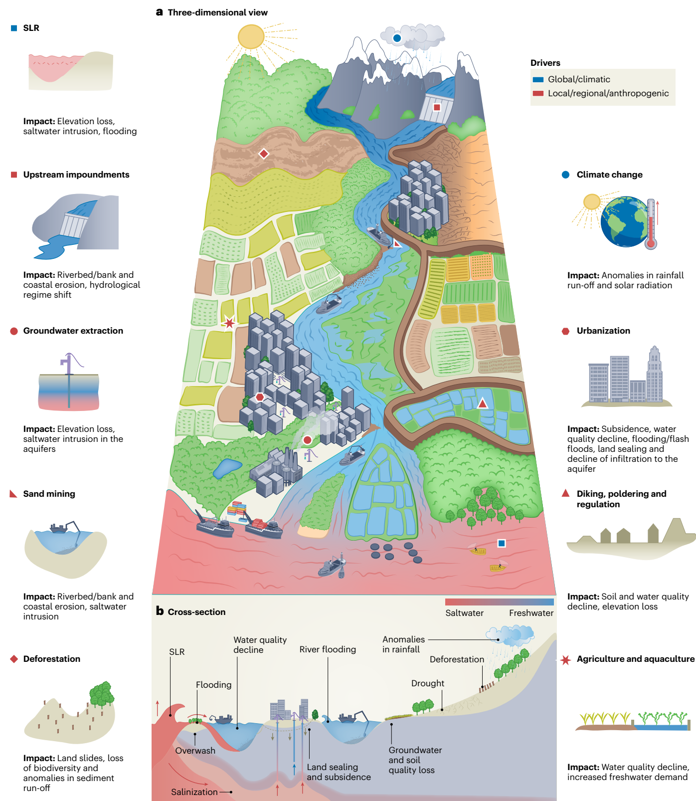
Fig. 1 | Climatic and anthropogenic drivers of change in the world's deltas. a, A three-dimensional view of the system. b, A conceptual cross-section from the sea to the mountains, featuring the surface and groundwater variability along the river. Credit: © Deltares: artwork by Dirma Janse.
